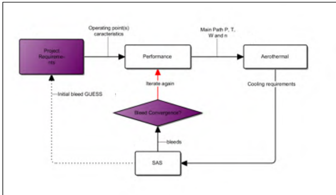
Figure 3.5 SAS-Performance-Aerothermal interconnectivity
