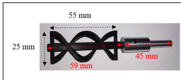
Figure 2.1 3D printed spindle into its shaft
