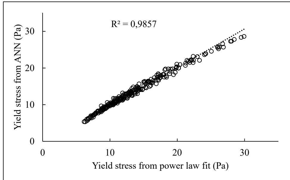
Figure 2.20 Correlation between yield stress from ANN (based on rheometer measurements) and from Power law fit with mini-slump
