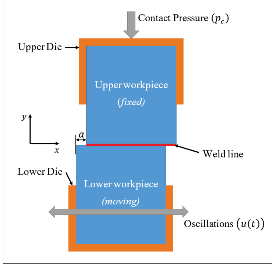
Figure 1.2 Vertical mounting setup of the linear friction welding
