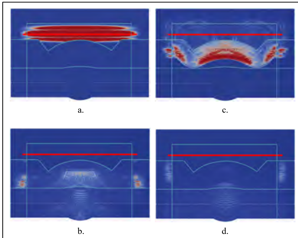
Figure 3.4 Wave propagation during a SAM measurement. a. Excitation. b. Focalization inside water. c. propagation inside the sample. d. Back propagation of signals towards the transducer
