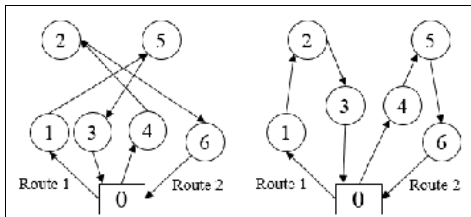
Figure 5.3 Inter-swap neighborhood
