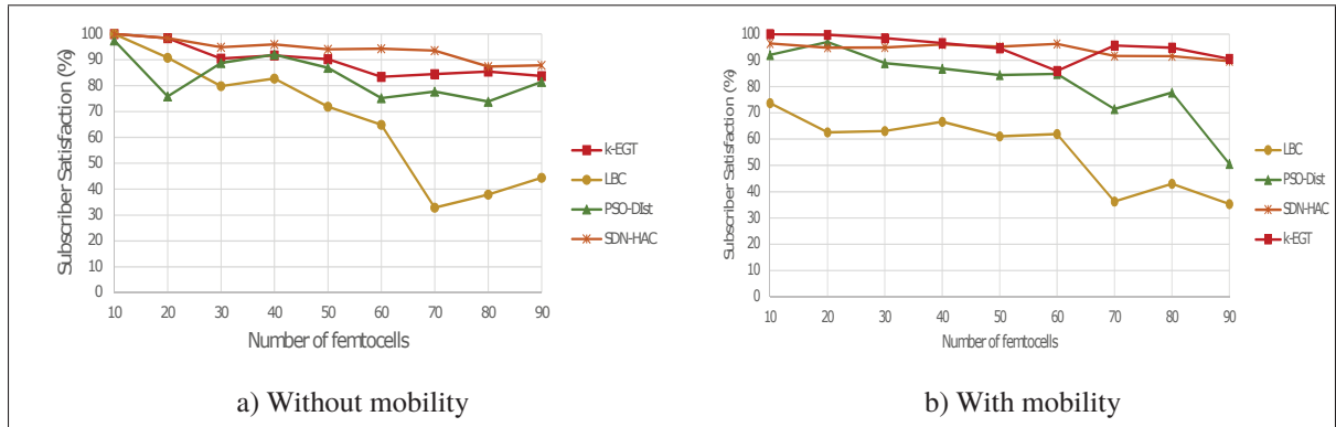
Figure 4.6 Subscriber satisfaction for dense-deployment of femtocells
