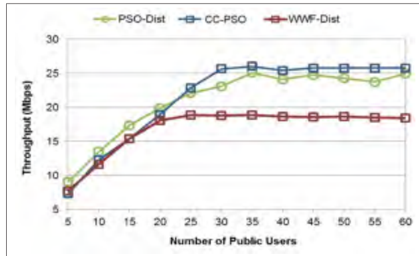
Figure 2.6 Network throughput
