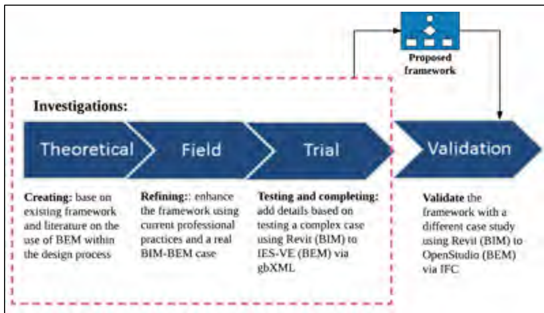
Figure 4.1 Research design
