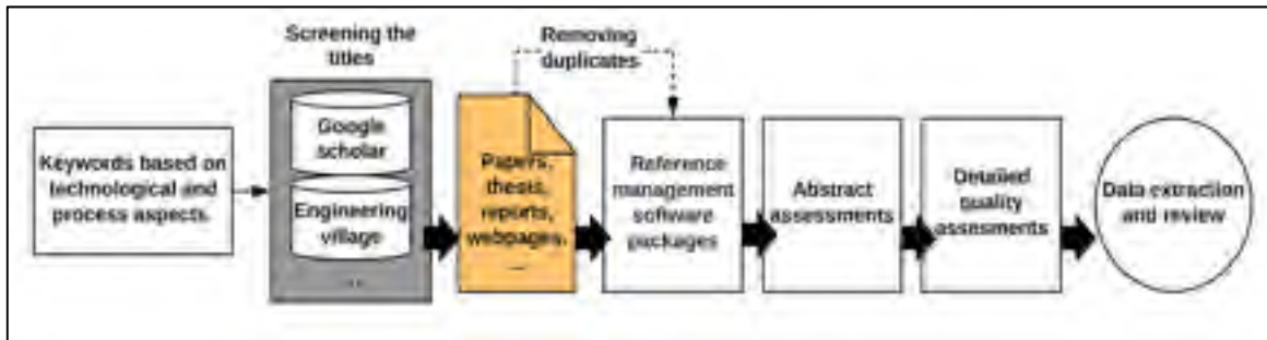
Figure 2.1 SLR procedure
