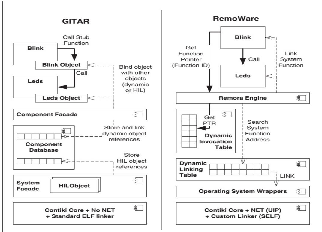
Figure 3.4 Comparison between Gitar and RemoWare
