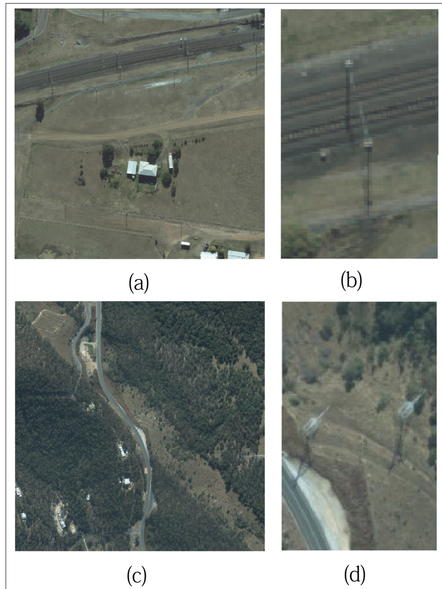
Figure 1.4 a) Rural area image with visible pole shadows around the dirt roads and rail tracks, b) Close up views of rail poles, c) Rural area image with electricity poles and pylons. d) Close up views of electricity poles or pylons. Reference: Pontecorvo & Redding (2017) page 5
