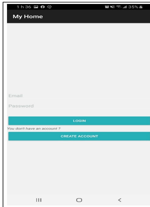
Figure 4-7 Interface 'Connexion'
