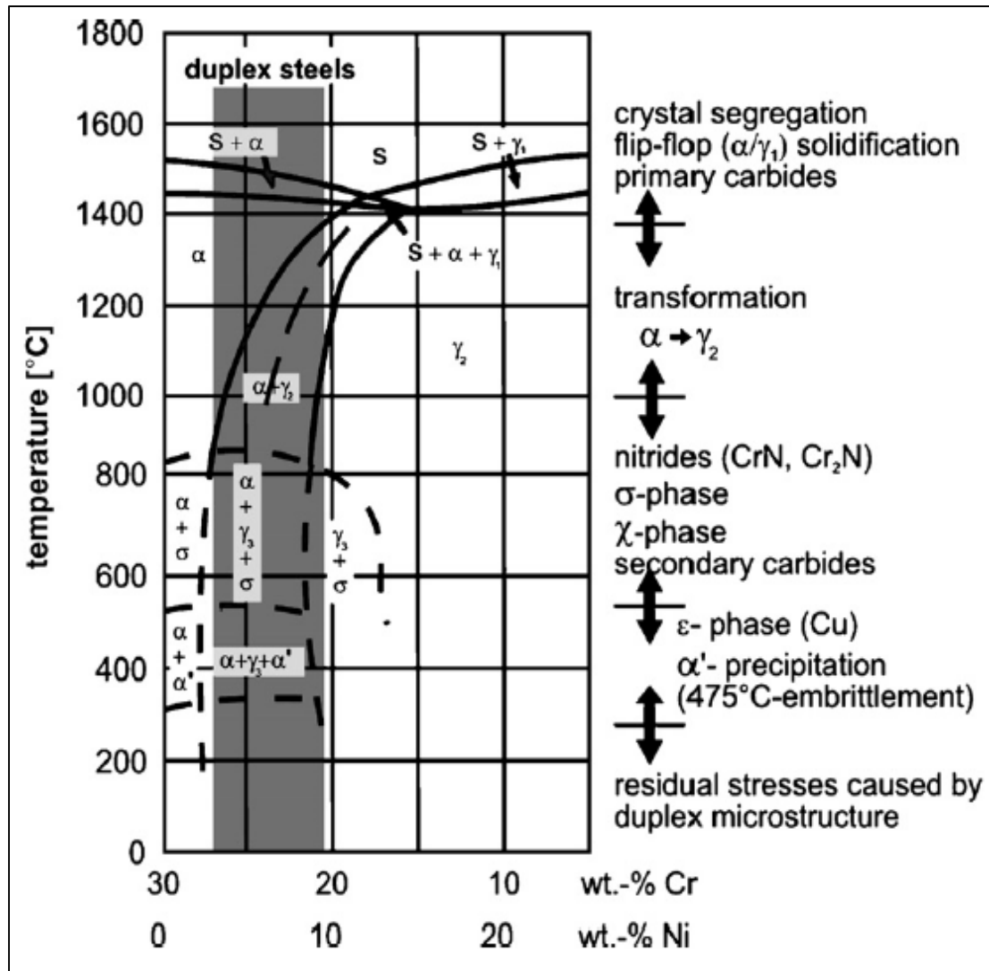
Figure 1.3 Diagramme pseudo-binaire 70Fe-Cr-Ni (Pohl, Storz et Glogowski, 2007)
