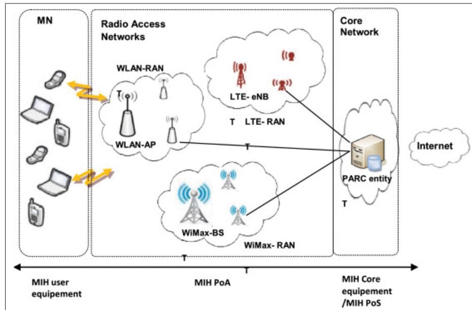
Figure 3.4 Proposed interworking architecture in Ali et al. (2018)
