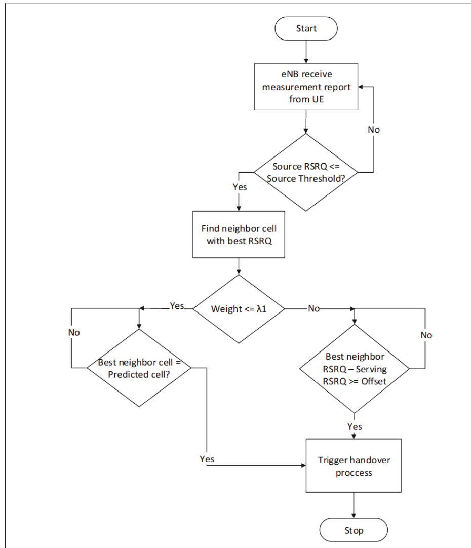
Figure 3.9 Vehicular Location Prediction Handover Algorithm (VLPFA) Hasbollah et al. (2017)
