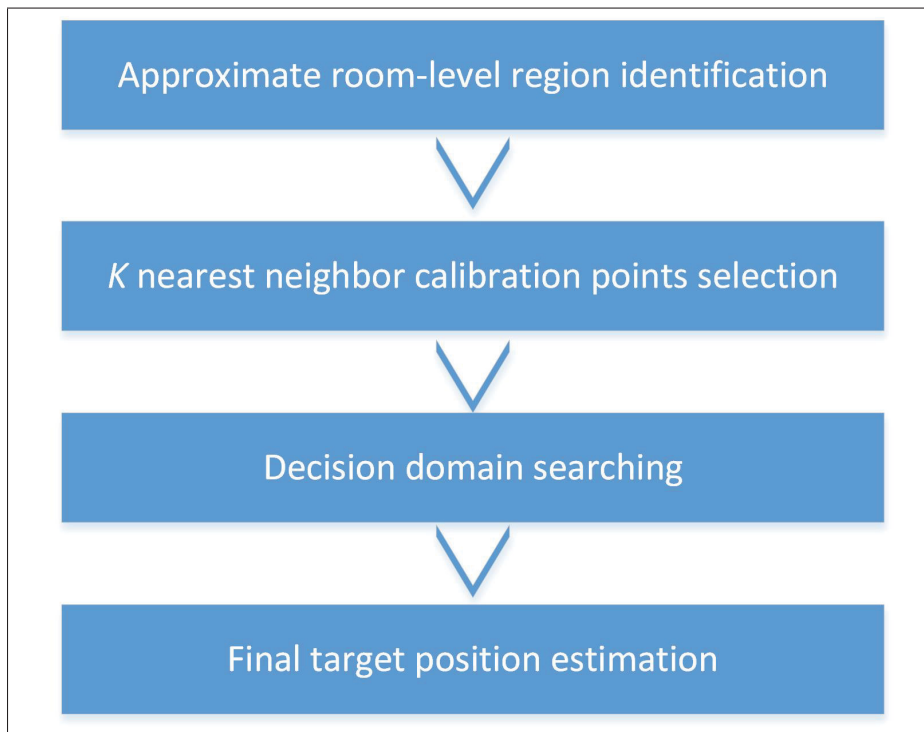
Figure 3.6 Flow chart of RDC (Desision Domain-based positioning) Zhang et al. (2017b)
