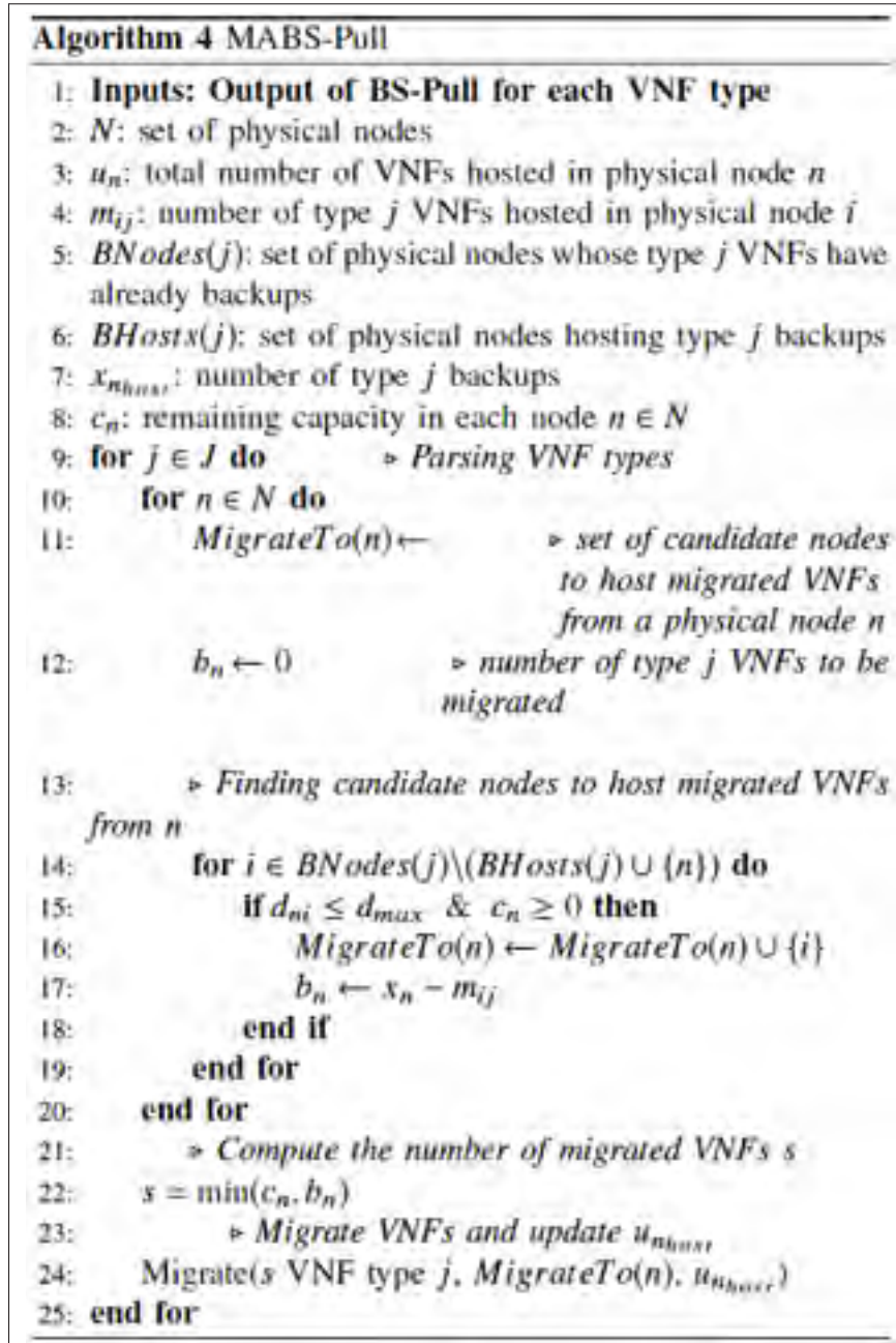
Figure 3.5 Algorithme MABS-Pull.
