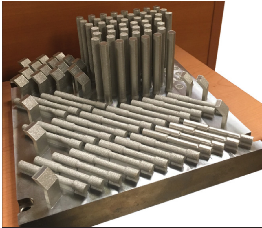
Figure A 2: Image of the build plate with 0° and 90°-oriented tensile blanks series
