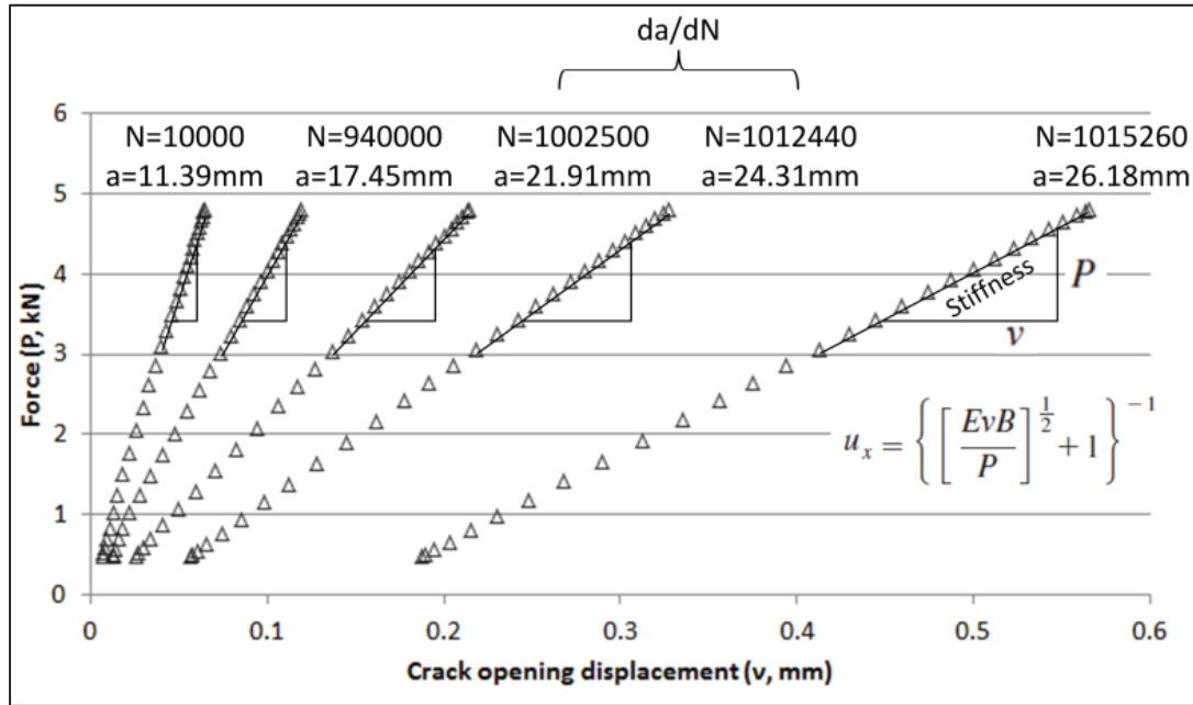
Figure 2.6 Typical stiffness curves ( v - P ) obtained for the fatigue crack growth test at SIFs ranges of \approx 12, 20, 30, 40 and 50 \text{ MPa}\cdot\text{m}^{1/2} ; results are from a 90^\circ -oriented HIP LPBF specimen
