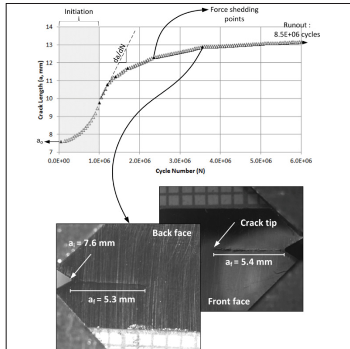
Figure 2.5 Schematization of the stepdown procedure preceded by the crack initiation procedure; results are from a 90°-oriented HIP LPBF specimen
