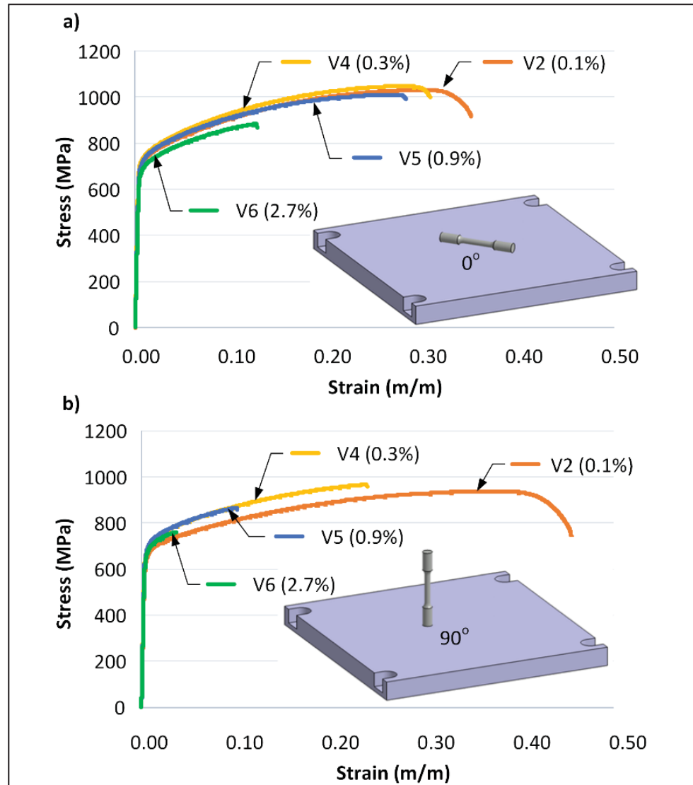
Figure 3.7 Typical tensile stress-strain diagrams obtained for the V2, V4, V5 and V6 parameter sets for the build orientations: a) 0° and b) 90°
