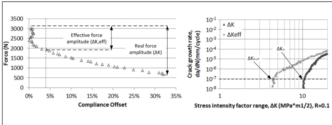
Figure 2.7 a) Compliance offset curve at a threshold for a specimen exhibiting crack closure at \approx 1900 N, b) Example of Paris curve using effective force amplitude ( \Delta K_{eff} ) compared to real force amplitude ( \Delta K ). Results are from a 90°-oriented HIP LPBF specimen.
