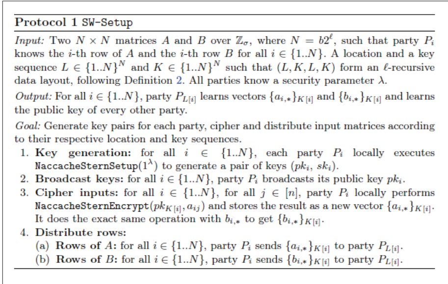
Figure 4.2 Initialization Phase of Strassen's Algorithm
