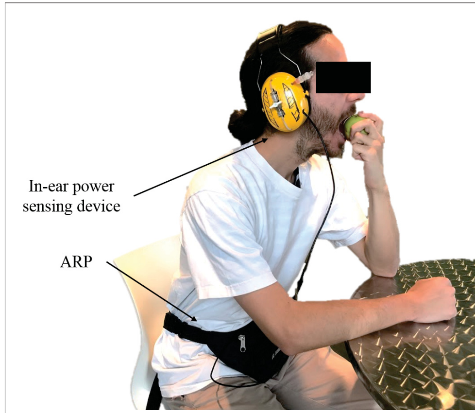
Figure 2.5 In-ear power sensing device in use while data is recorded by ARP placed inside a waist pack
