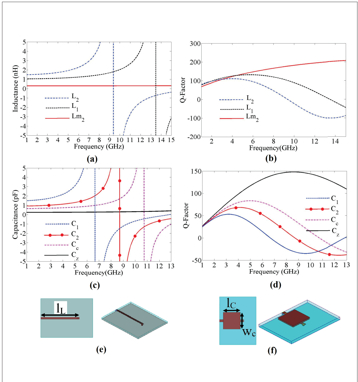
Figure 3.4 Simulated characteristics of elements in the HFSS a) simulated inductances of L_1 , L_2 and L_{m2} versus frequency b) simulated Q-factors of L_1 , L_2 and L_{m2} versus frequency c) simulated capacitances of C_1 , C_2 , C_z and C_c versus frequency d) simulated Q-factors of C_1 , C_2 , C_z and C_c versus frequency e) top view and 3D view of straight line inductor f) top view and 3D view of parallel plate capacitor
