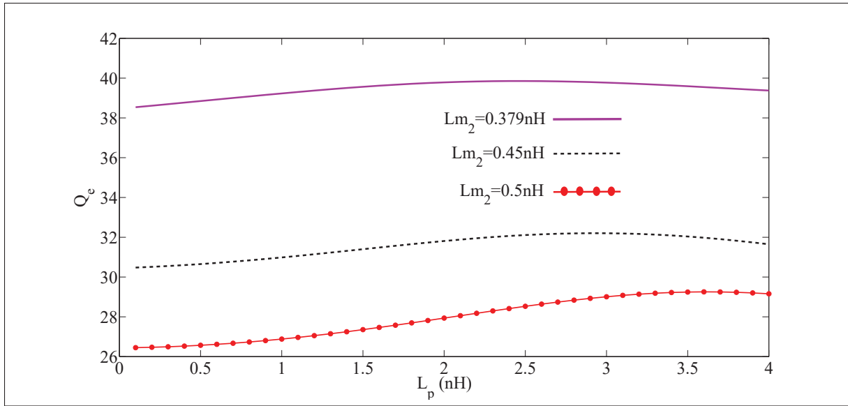
Figure 2.4 Variation of L_p versus Q_e
