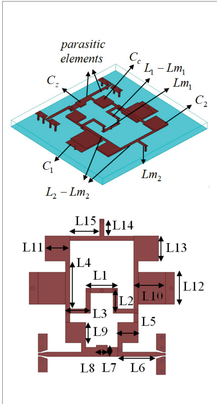
Figure 3.5 3D and top views of structured initial EM circuit in HFSS. Dimensions are in millimeters, L1=1.4 , L2=1.1 , L3=1.1 , L4=2.3 , L5=0.9 , L6=1.5 , L7=0.5 , L8=0.5 , L9=0.9 , L10=1.4 , L11=1.1 , L12=1.4 , L13=1.1 , L14=0.75 , L15=1.3 , width of lines=0.2
