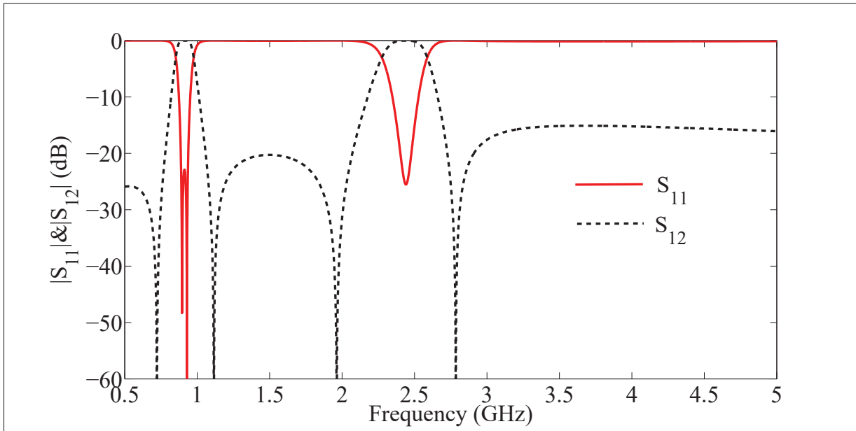
Figure 1.11 Simulated S-parameter of modified D-BPF circuit model with C_z = 0.2 pF
