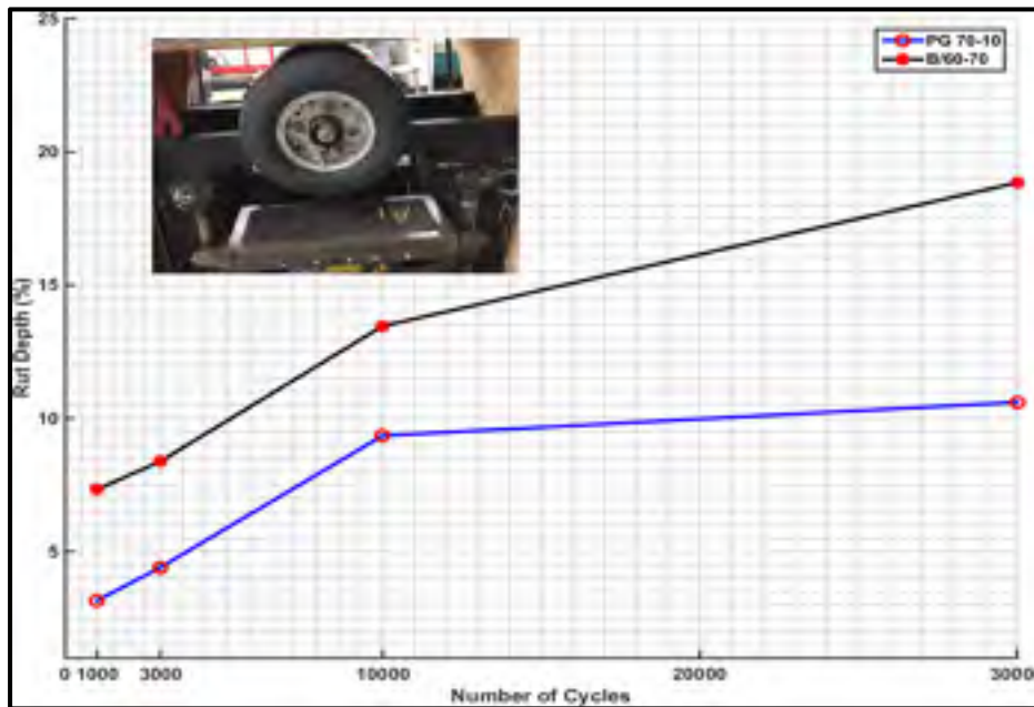
Figure AI. 6 Rutting results
