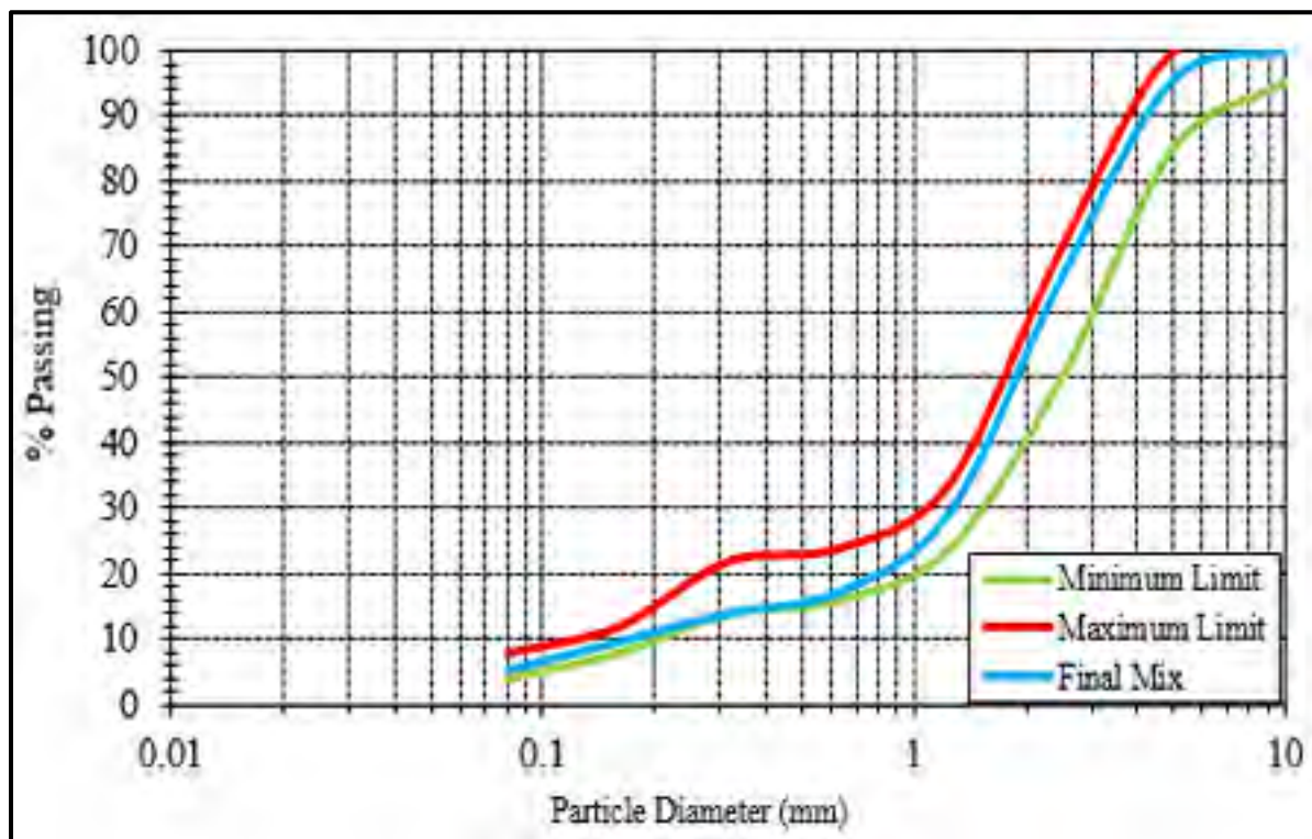
Figure 5. 4 Aggregates Gradation
