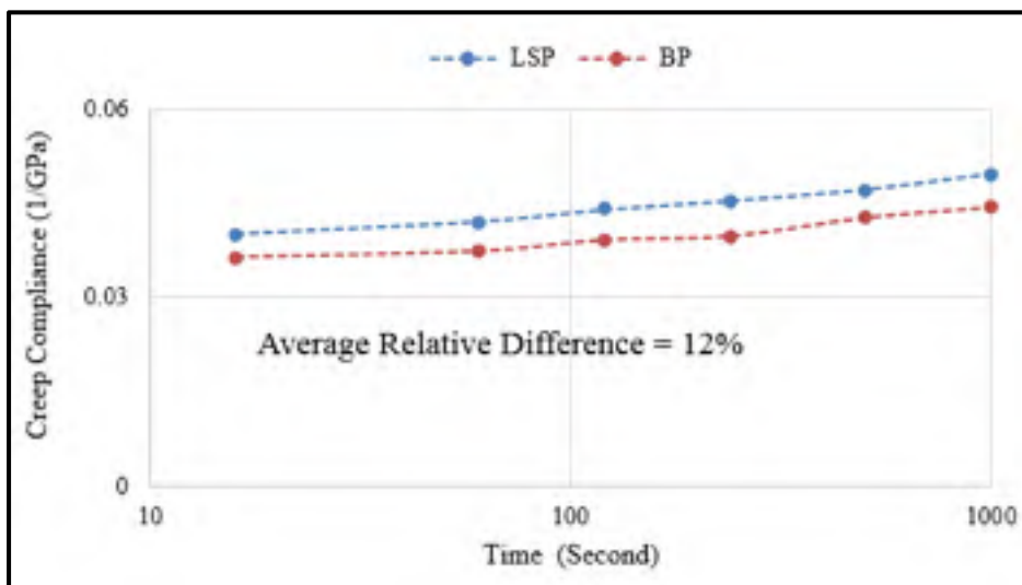
Figure 5. 15 Creep Compliance Comparisons, 0°C
