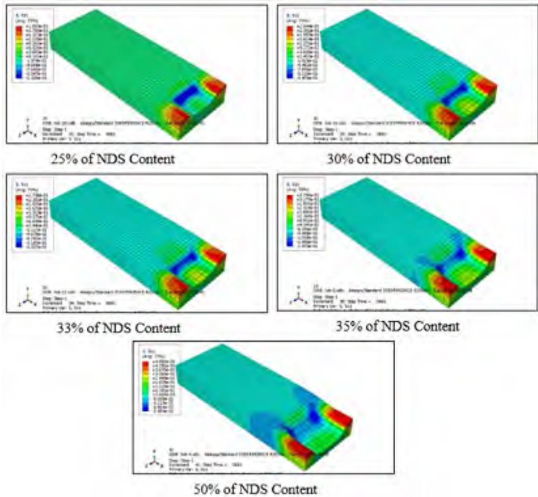
Figure 2. 1 Rut depth deformation after loading
