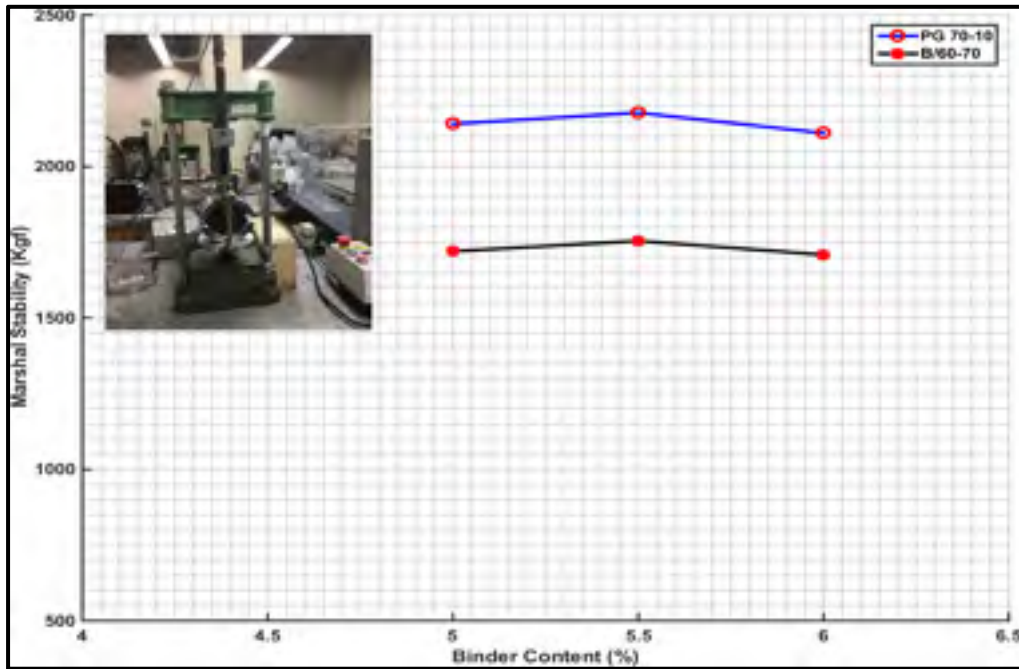
Figure AI. 4a Marshal stability
