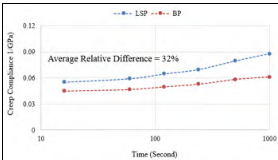
Figure 5. 16 Creep Compliance Comparisons, 20°C
