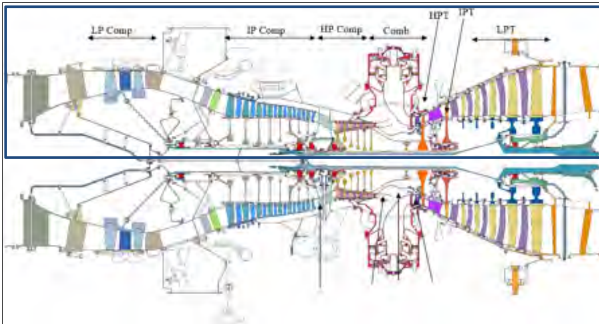
Figure 2.2 Cross section of a gas turbine
