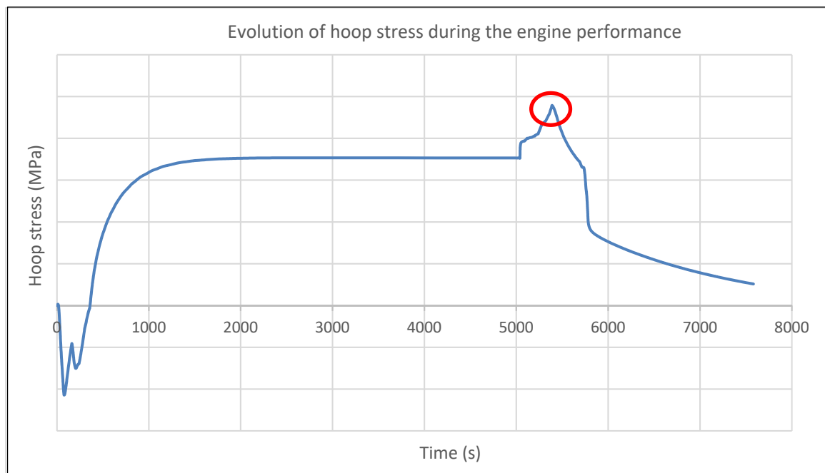
Figure 4.9 Hoop stress plot
