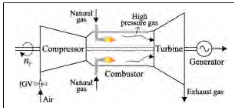
Figure 2.1 Gas turbine system diagram
