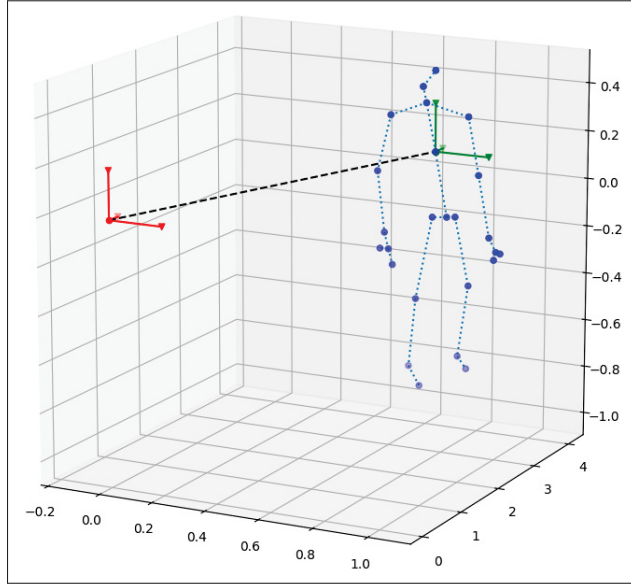
Figure 3.3 In red the coordinate system of the camera, in green the new coordinate system corresponding to the middle of the spine of the main subject for the first frame of the sequence, in blue the skeleton of the main subject, in black the translation vector
