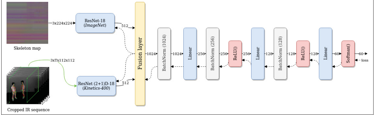
Figure 3.7 The full detailed model. The pose and IR modules output separate feature vectors. The two are fused (average, sum, multiplication, max, convolution or concatenation) and a final MLP outputs a class probability distribution. The pose network is a pre-trained ResNet-18 . The IR network is a pre-trained network R(2+1)D-18
