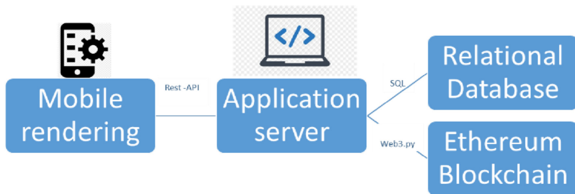
Figure 6.4: Application layer
