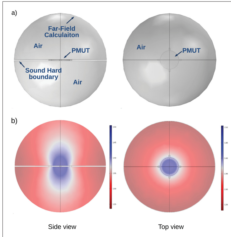
Figure 5.4 COMSOL simulation. a) model used for simulation and b) simulation results of acoustic pressure level in dBV
