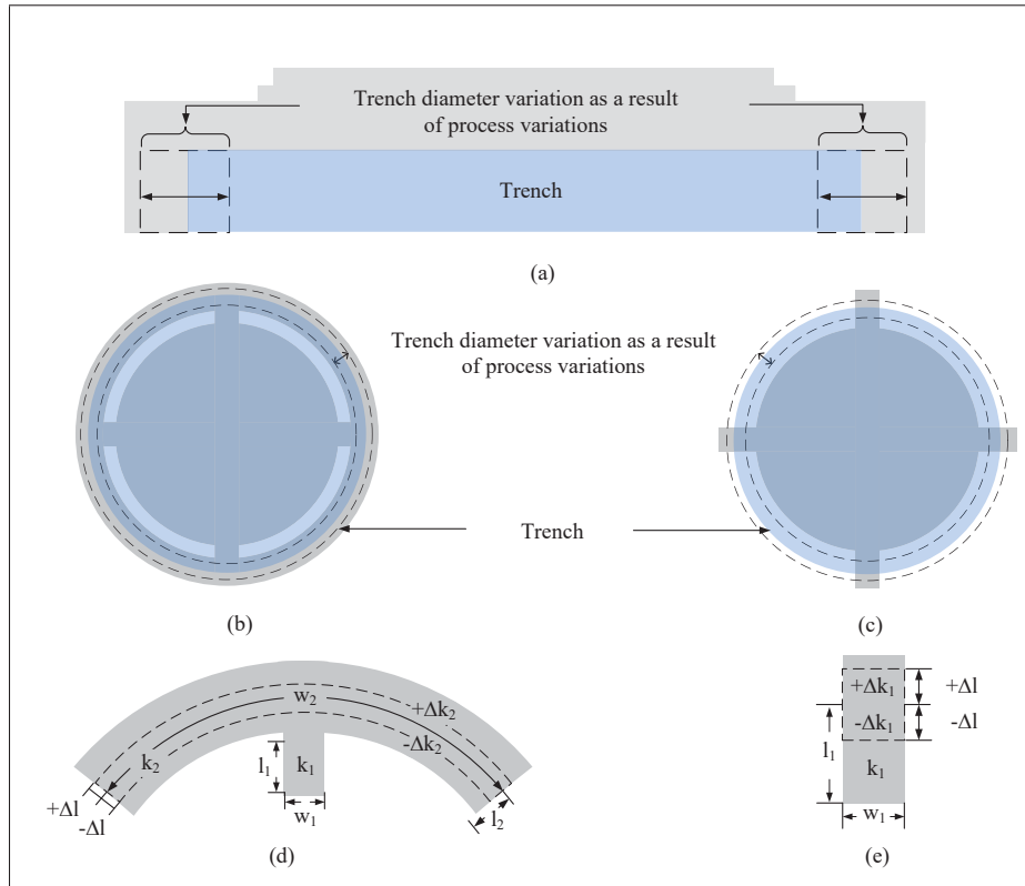
Figure 3.1 Schematic of a PMUT with toroid anchor ; (a) Cross view of the PMUT with toroid anchor with the designation of the trench and its variation as a result of process variations. (b) Top view of the PMUT with toroid anchor with the designation of the section illustrated in (d). (c) Top view of the PMUT without toroid anchor with the designation of the section illustrated in (e). (d) Anchor section of the PMUT with toroid and identification of the spring constant, length and width and their variations. (e) Anchor section of the PMUT without toroid and identification of the spring constant, length and width and their variations
