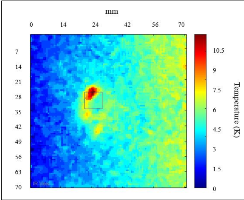
Figure 2-15 E3 raw thermogram at t = 0.66\text{s}
