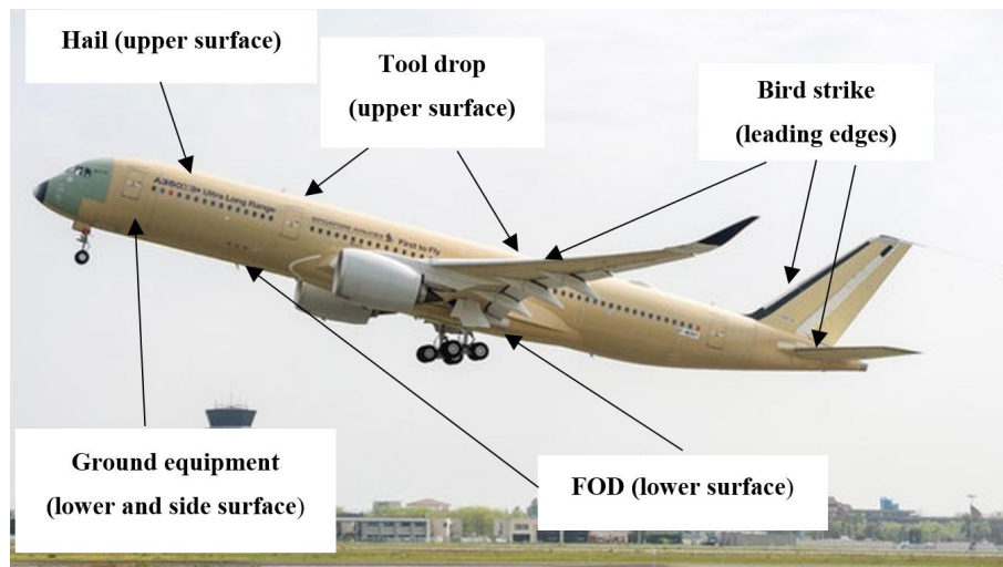
Figure 1-2 Impact damage scenario
