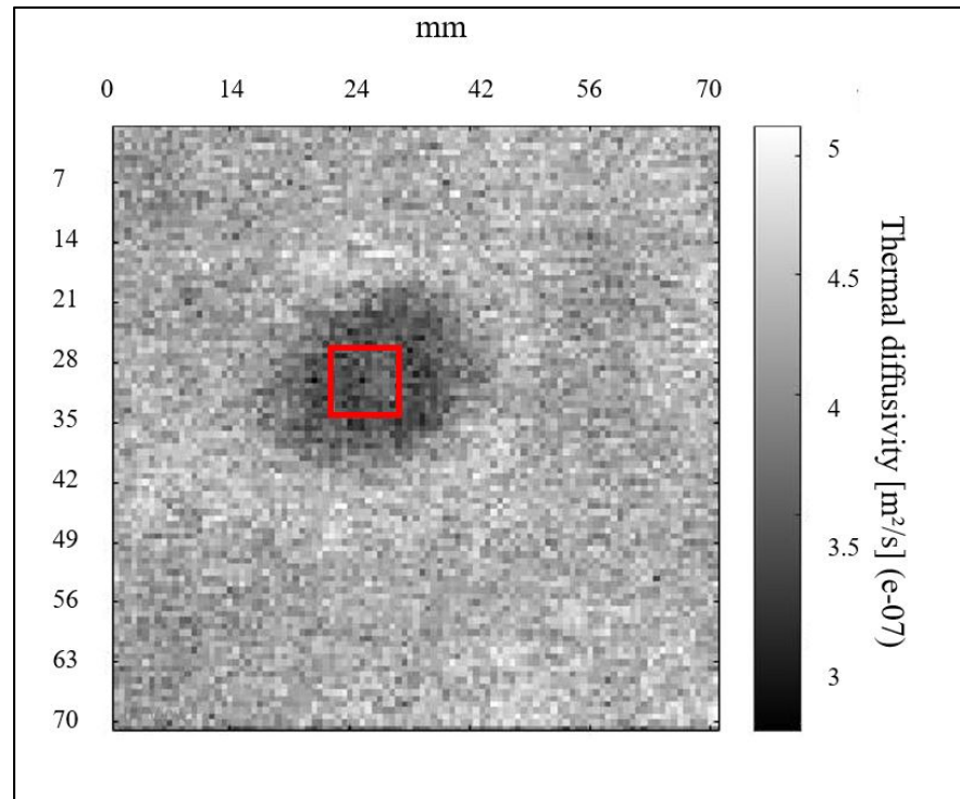
Figure 2-24 E2, diffusivity map
