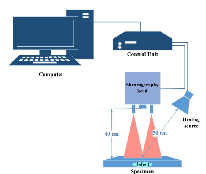
Figure 3-6 Shearography setup
