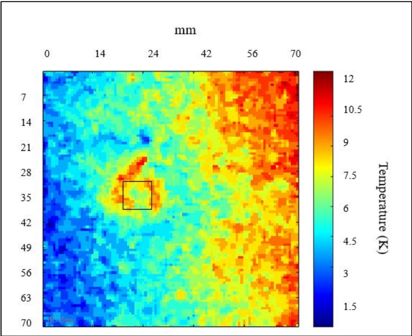
Figure 2-14 E2 raw thermogram at t = 0.66\text{s}
