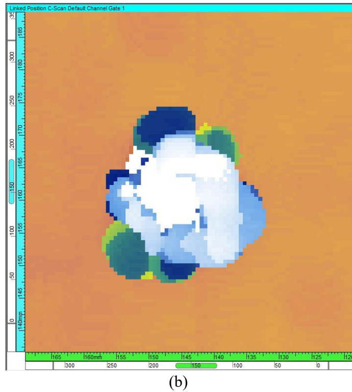
Figure 1-14 E4, C-scan of the defect from the (a) tool and (b) bag side
