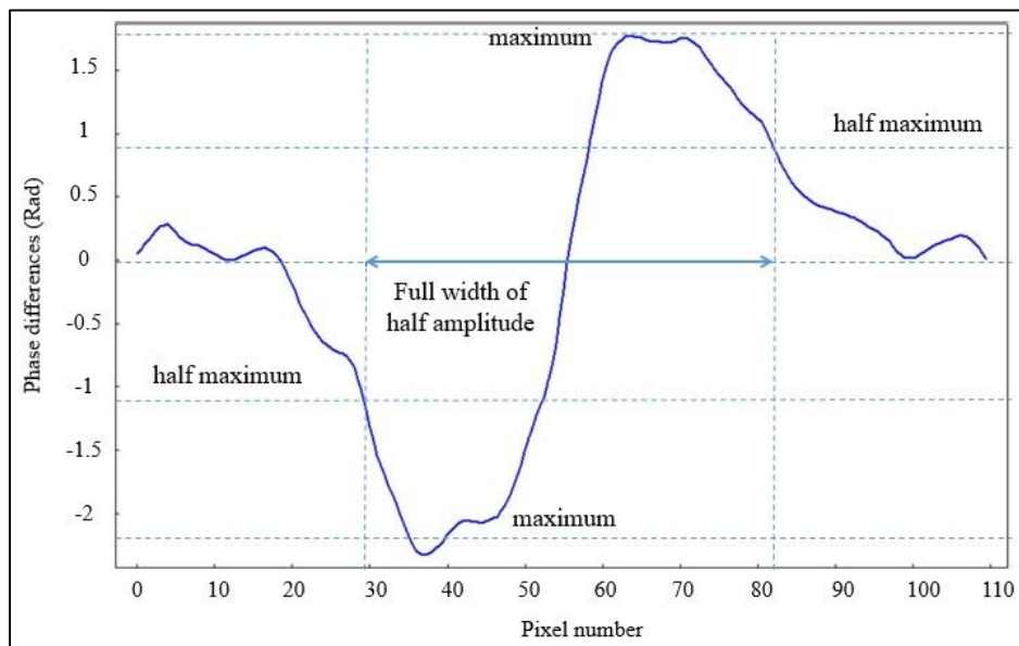
Figure 3-15 E3, indication sizing by full-width of half-amplitude
