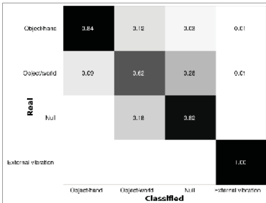
Figure 3.14 Confusion matrix
