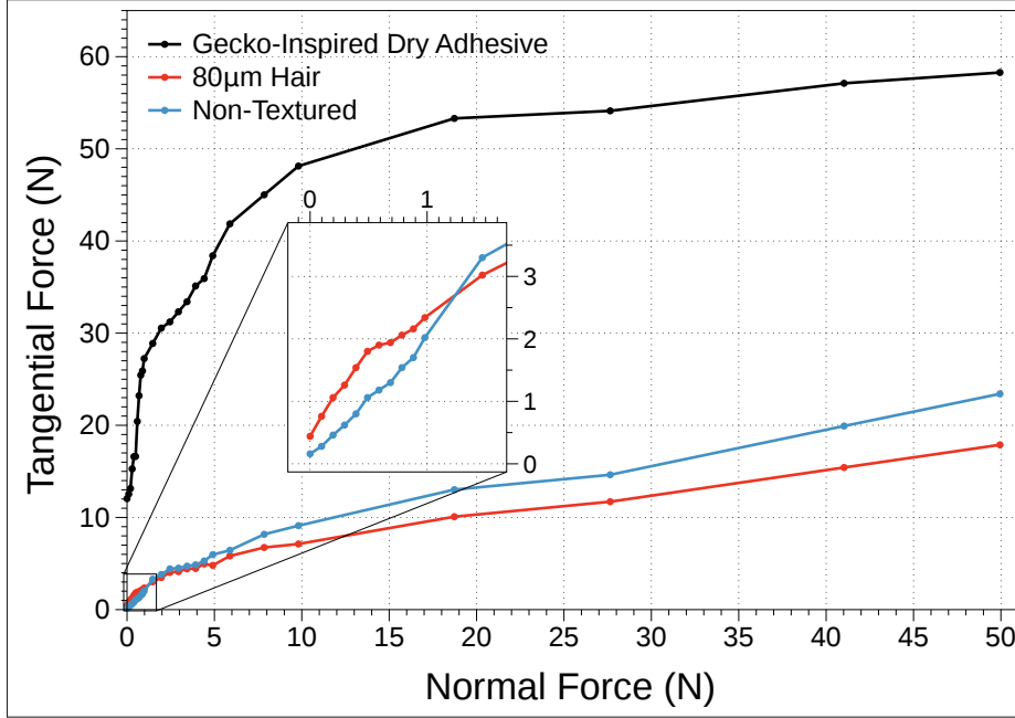
Figure 2.5 Comparison of maximum tangential force, F_{t,max} as a function of normal force for 31 mm 2 samples of (i) gecko-inspired directional adhesives pulling in the preferred direction, (ii) a texture of non-directional silicone hairs (fig. 2.4), and (iii) flat silicone PDMS
