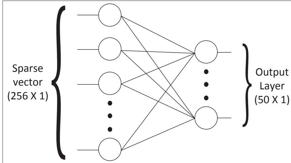
Figure 4.4 The two sparse vectors (128 elements each) are concatenated and linked to a simple fully-connected layer with 50 output nodes, where each node correspond to a specific object (here, the 128 elements are due to the 128 features contained in the dictionary, see Roberge et al. (2016))
