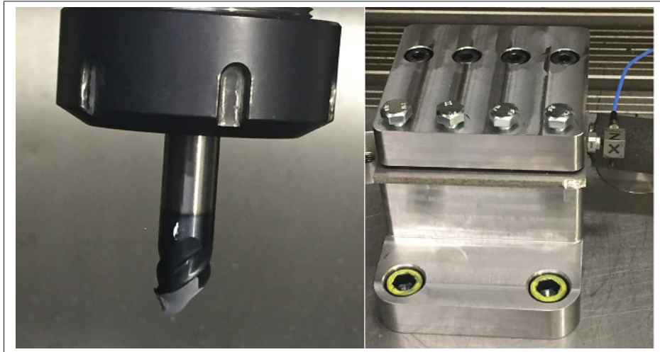
Figure 2.7 Tool breakage due to uneven surface of the workpiece in first path
