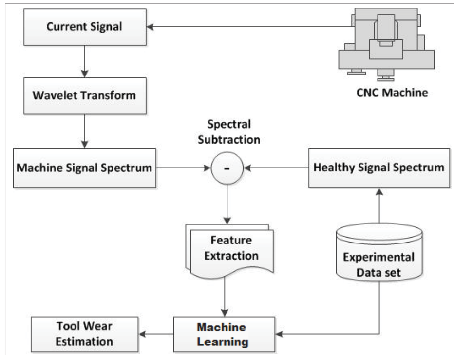
Figure 3.1 Methodology diagram
