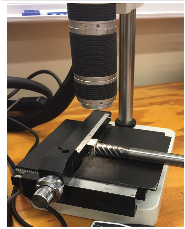
Figure 2.8 Keyence microscope used for tool wear measurement
