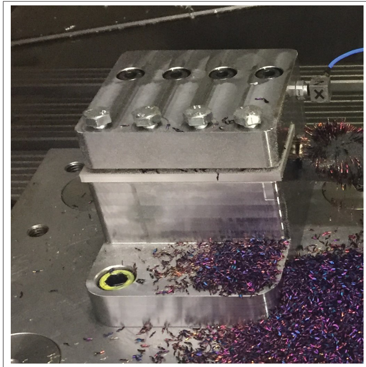
Figure 2.6 Jig designed for holding the work piece in place
