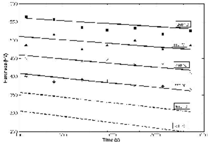
Fig. 4. Hardness during tempering treatment of AMS 6414
