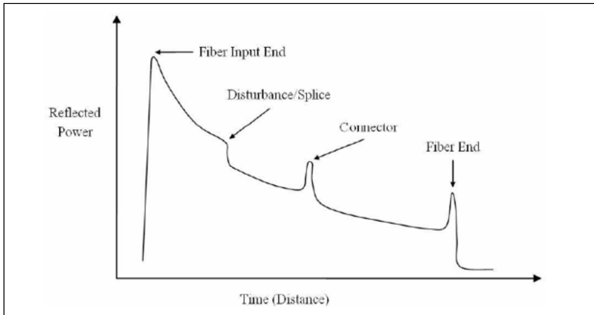
Figure 3.26 Trace OTDR typique (Park, 1992)
