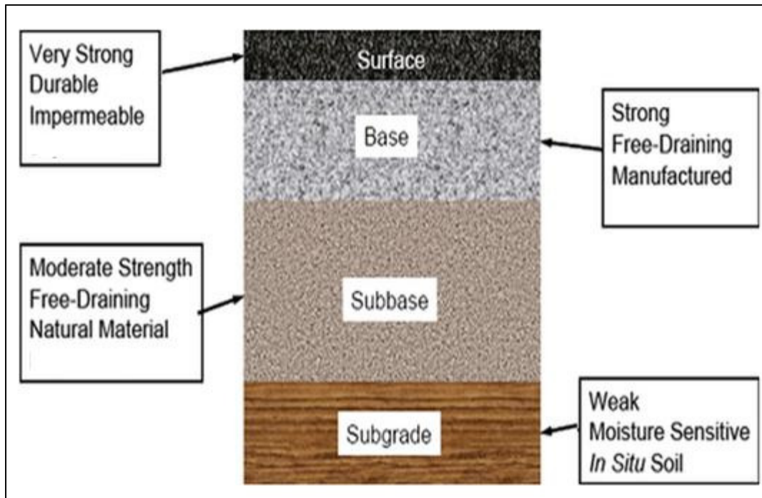
Figure 2.4 Structure de la route (FHWA, 2007)
