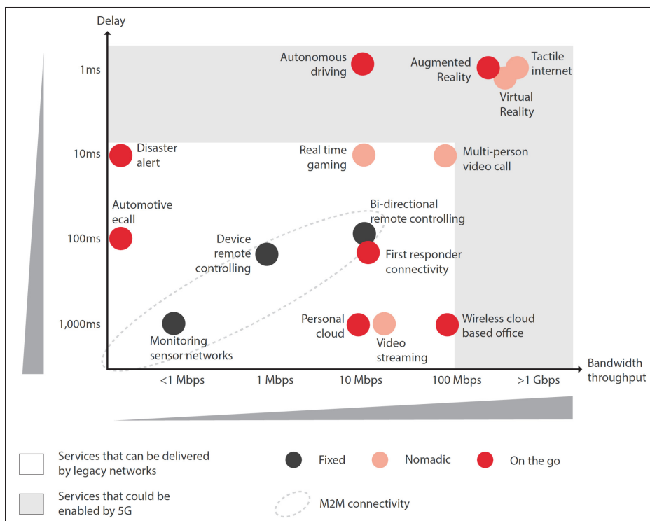
Figure 1.1 Potential 5G use cases and their bandwidth / latency requirements Taken from Intelligence (2014)
