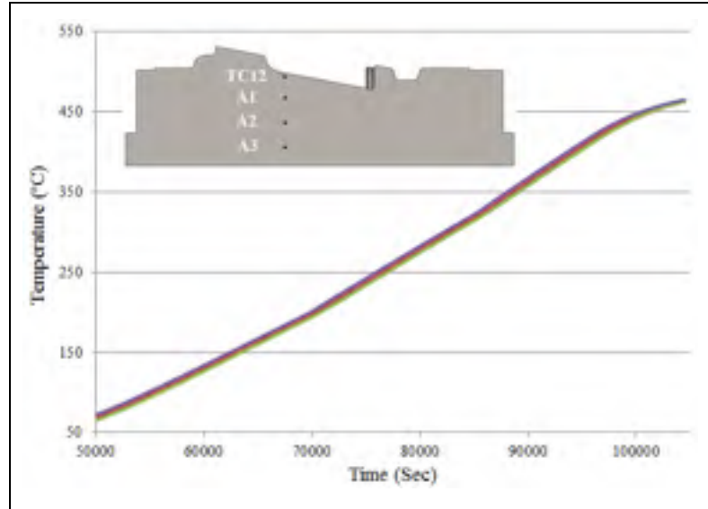
Figure 2-12 The temperature evolution comparison between TC12 and the points inside the die as A1, A2 and A3.
