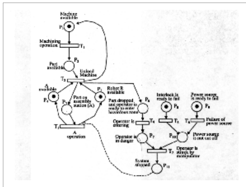
Figure 1.4 Fault Petri net example (Source: Adamyian and He, 2002)
