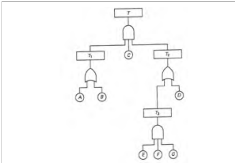
Figure 3.1 An example of a fault tree
