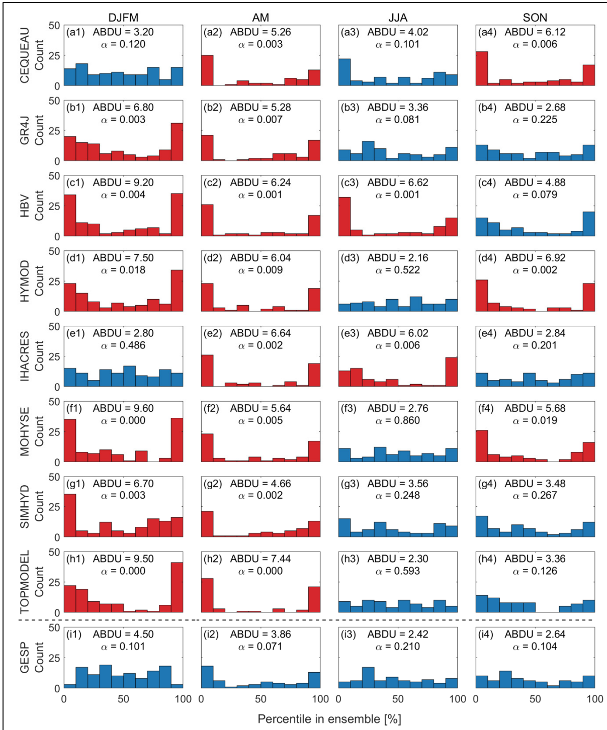
Figure 2.4 Talagrand diagrams representing rank (in percentiles) occupied by observed streamflows in the ESPs of eight different hydrological models after performing DA and QM on the LSJ catchment. Blue (red) diagrams indicate that the K-S test failed to reject (rejected) the hypothesis of uniformity ( \alpha = 0.05 )
