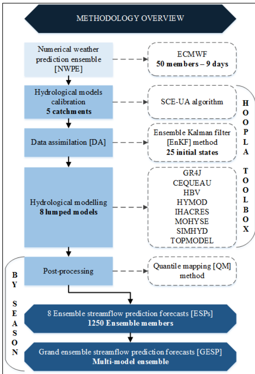
Figure 2.2 Proposed methodology implemented in this study
