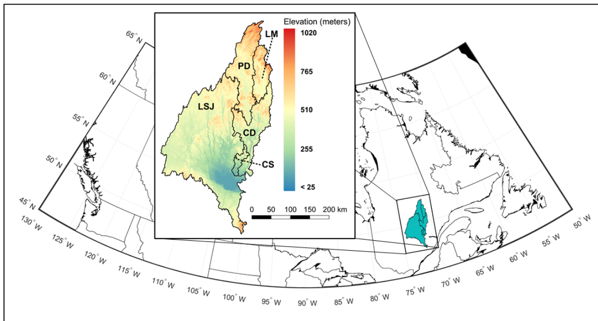
Figure 2.1 Location and topography of the study's five catchments
