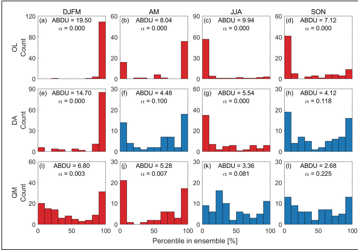
Figure 2.3 Talagrand diagrams representing rank (in percentiles) occupied by observed streamflows in the hydrological forecast ensemble using the GR4J model on the LSJ catchment. “OL” refers to the open-loop simulation. “DA” refers to the validation members of the 1250 ensemble members after performing data assimilation and “QM” refers to the same members after performing data assimilation and post-processing with quantile-mapping. Blue (red) diagrams indicate that the K-S test failed to reject (rejected) the hypothesis of uniformity ( \alpha = 0.05 )
