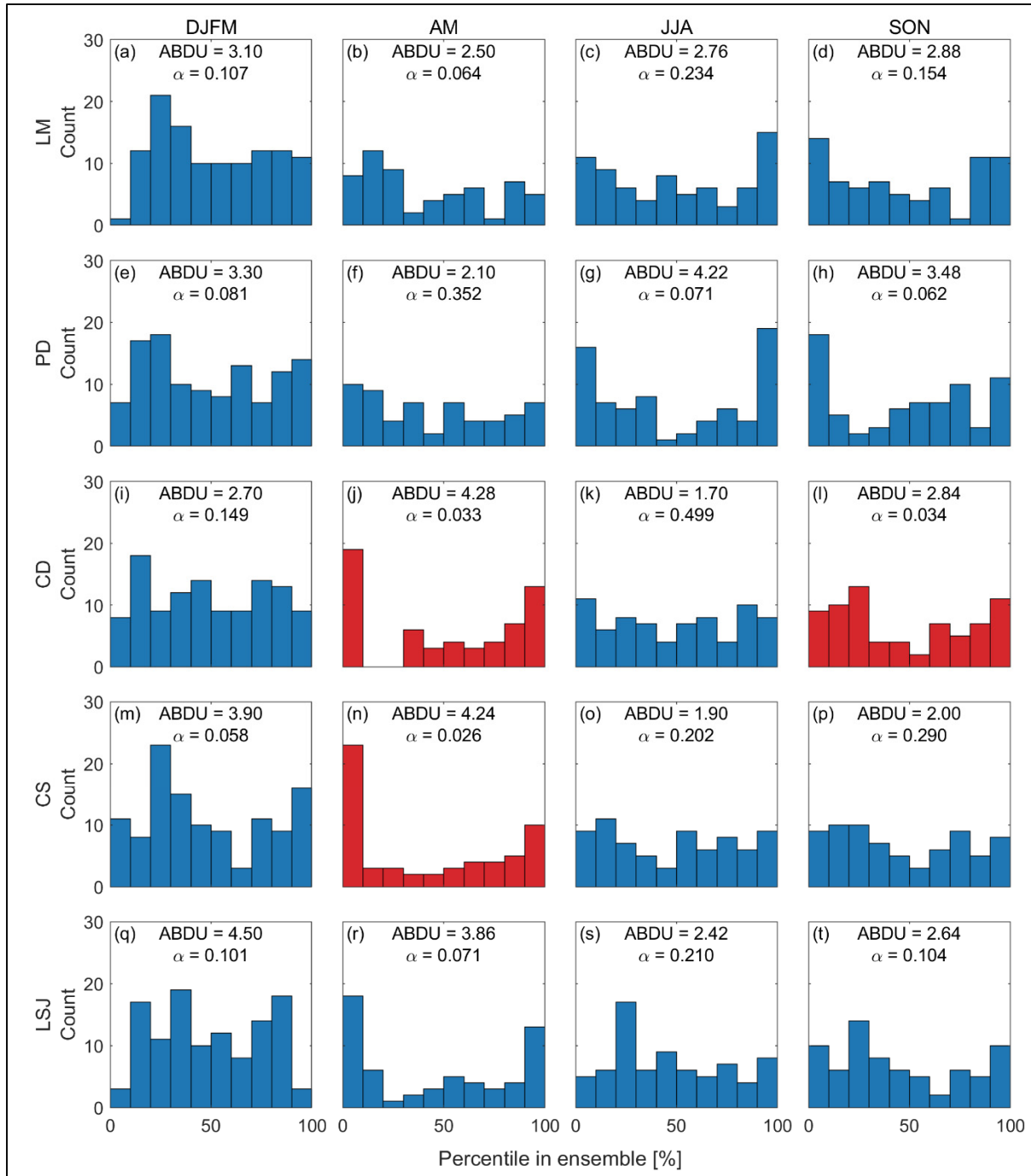
Figure 2.5 Talagrand diagrams representing rank (in percentiles) occupied by observed streamflows in the hydrological multi-model (GESP) forecast after performing DA and QM on the five catchments. Blue (red) diagram indicates that the K-S test failed to reject (rejected) the hypothesis of uniformity ( \alpha = 0.05 )
