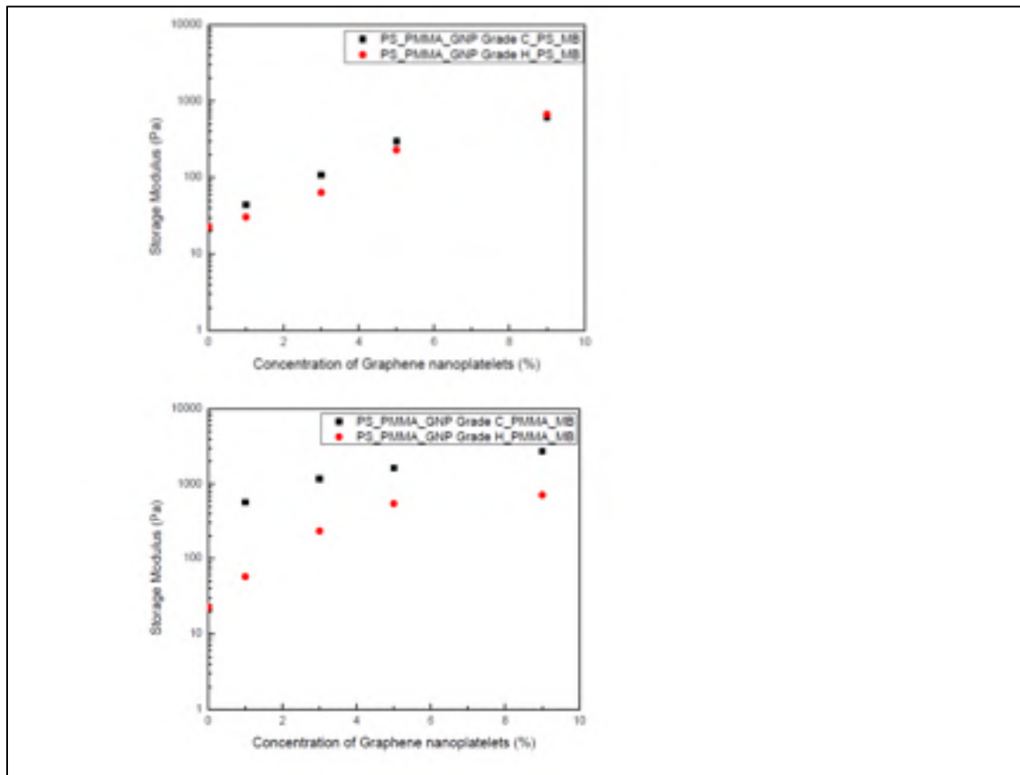
Figure 4.11 Rheological percolation taken at 0.01 rad/s as a function of graphene concentration for different composites prepared from a)PSMB b)PMMAMB
