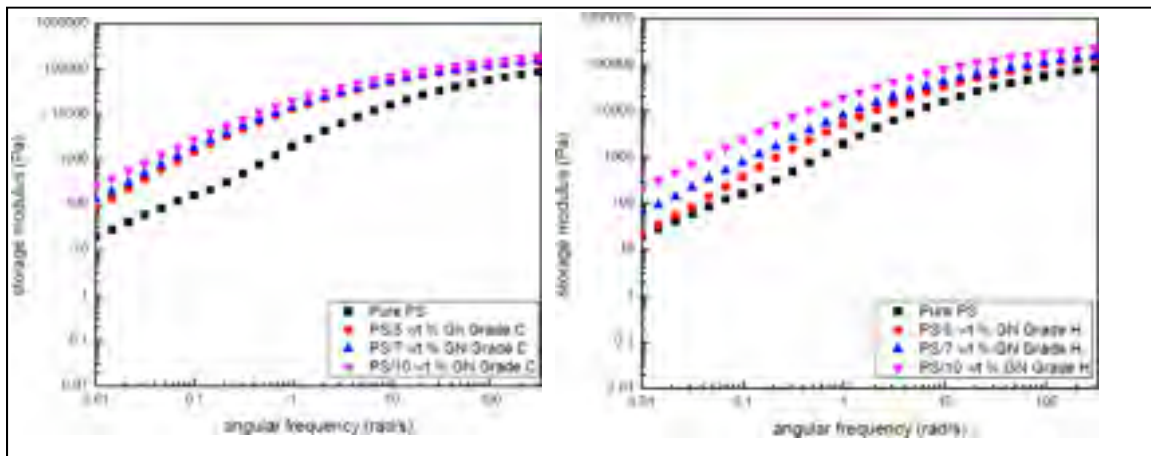
Figure 4.2: Storage modulus as a function of angular frequency for a)PS filled with grade C b)PS filled with grade H
