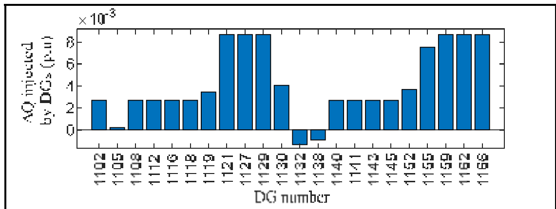
Figure 5.7 The total compensated reactive power outputs by DGs for scenario 1
