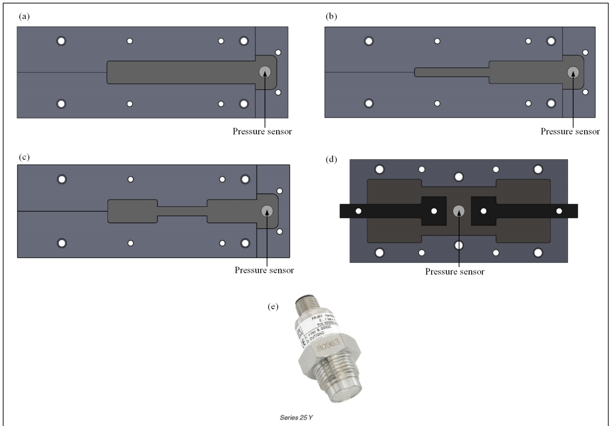
Figure 3.7 (a-d) Top view of the mold cavity with pressure sensor positions, and (e) image of the piezoresistive pressure sensor (series 25Y)
