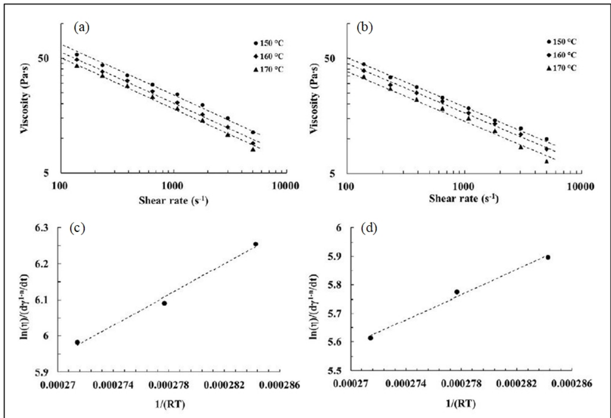
Figure 1.4 (a-b) Viscosity profiles and fitting results (the slope of dash line is n value) for 67 vol. % Ti feedstock and 64 vol. % BE Ti64 feedstock at three different temperatures respectively (c-d) Flow activation energy represented as the slopes of linear fit for 67 vol. % Ti feedstock and 64 vol. % BE Ti64 feedstock respectively
