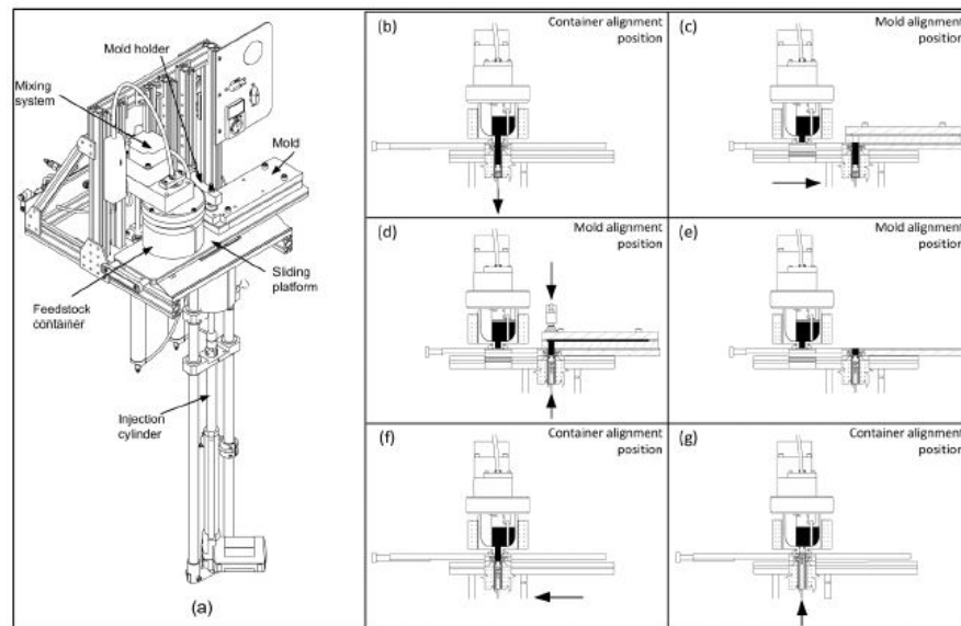
Figure 3.6 (a) General view of the injection system in a mold Alignment position, and (b-g) partial section views of the injection system describing the method for injecting a feedstock Taken from Lamarre (2016, p. 52)
