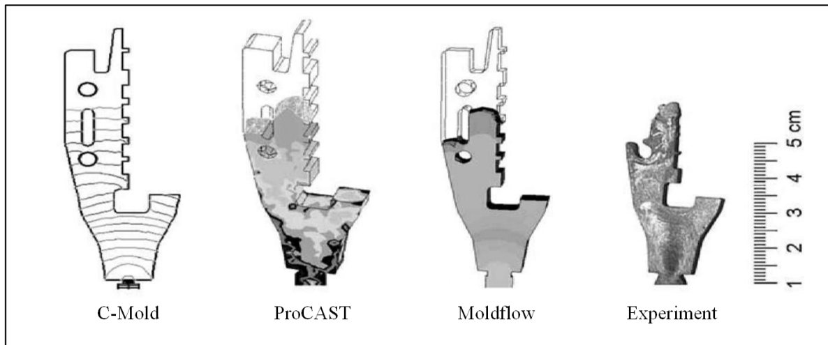
Figure 1.13 Simulated filing patterns compared to experimental result
