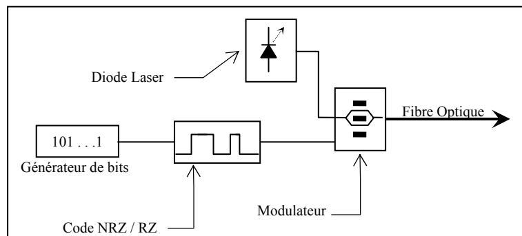
Figure 1.4 La modulation externe.
