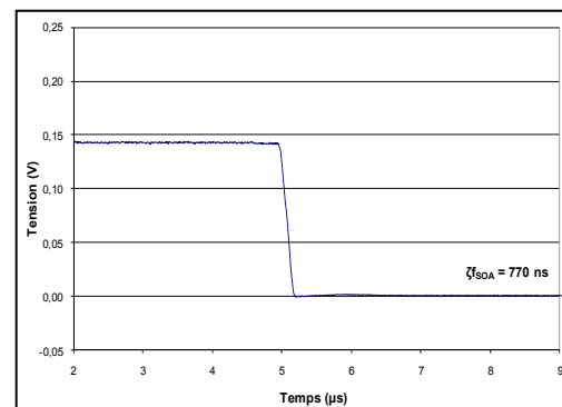
Figure 2.35 Tracé descente à 1μs (cas C).
