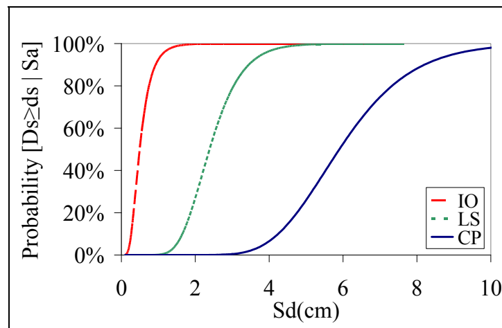
Figure 4.9 Displacement-based fragility curves for the CIW building at the three performance levels.
