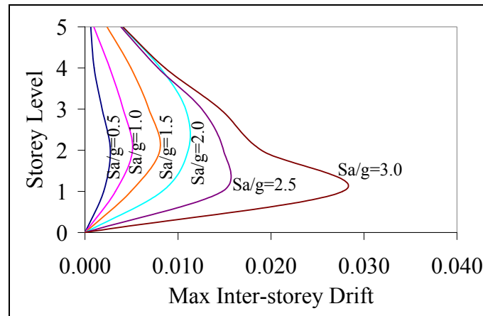
Figure 5.5 CIW's maximum ISD of all storeys at different values of S_a(T_x) for group 5 of the ground motion in Table 3.8.
