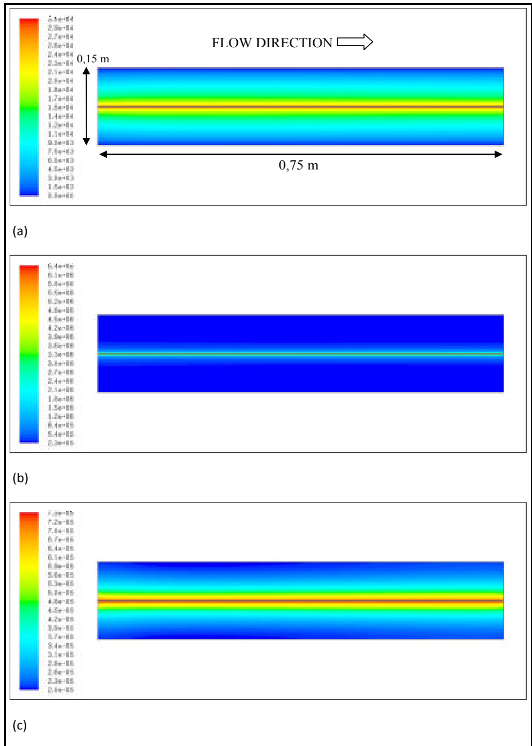
Figure 3.10 Electrostatic variables for the reference model simulation: (a) Electric potential (V), (b) Electric field strength (V/m), (c) Ion charge density ( \text{C/m}^3 ).
