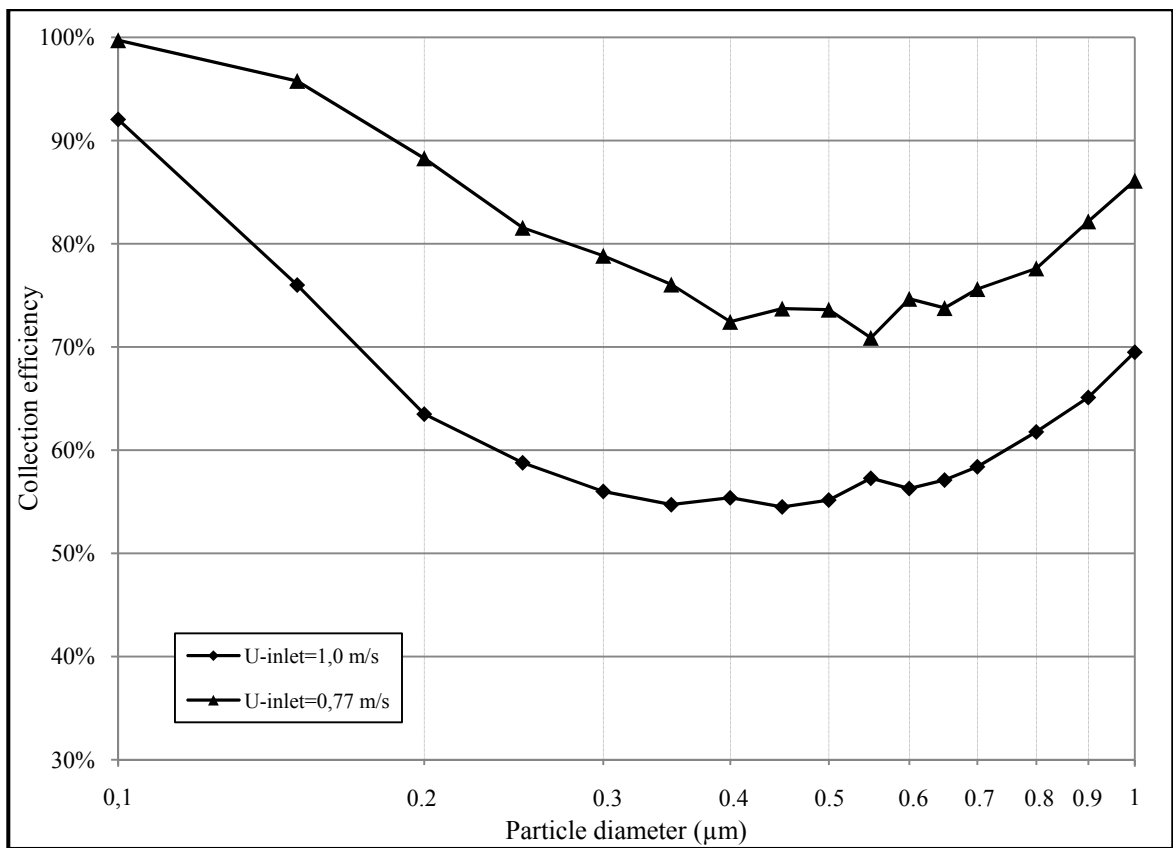
Figure 3.19 The ESP collection efficiency curve as obtained from the prototype model simulation for two inlet gas flow velocities.
