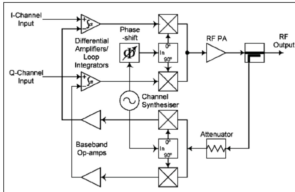
Figure 1.8 La technique Cartesian Feedback.
