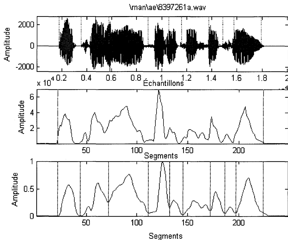
Figure 48 Segmentation en syllabes sans correction
