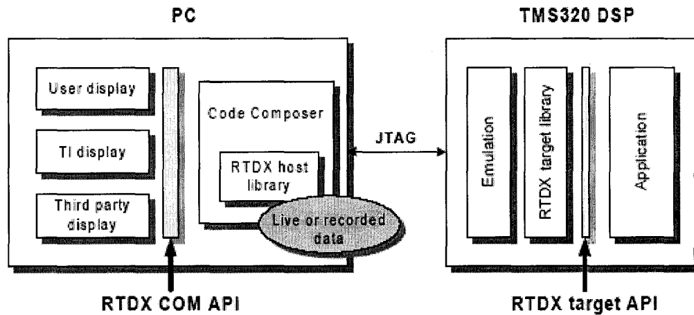
Figure 35 L'outil JTAG [57]
