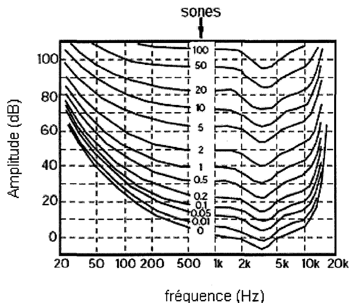
Figure 8 Courbes isosoniques [13]
