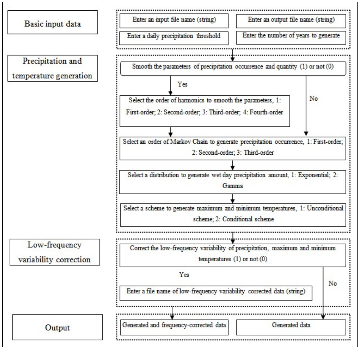
Figure 3.1 Structure chart of the WeaGETS stochastic weather generator.
