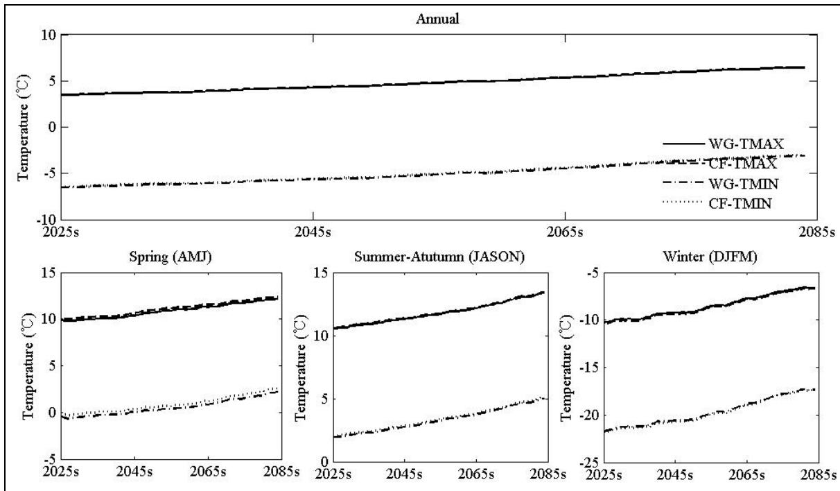
Figure 6.8 Annual and seasonal Tmaxs and Tminns downscaled by change factor (CF) and weather generator-based (WG) methods over the 2025-2084 period for the Manicouagan 5 river basin.
