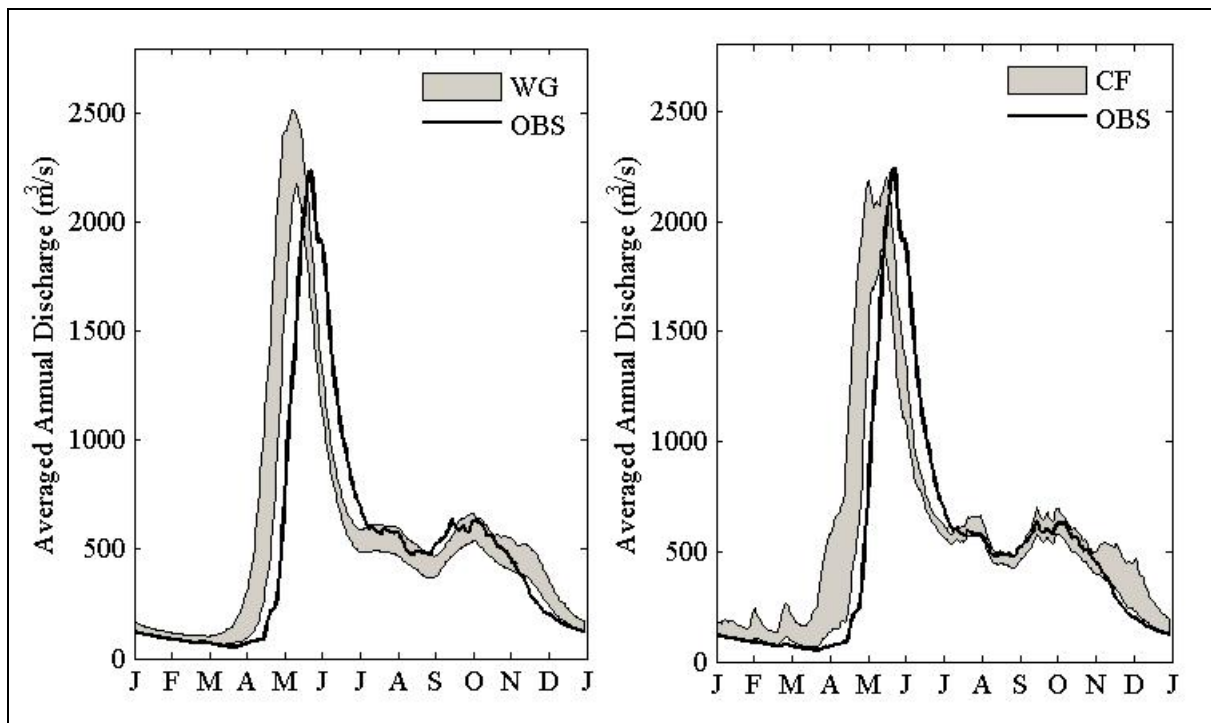
Figure 6.13 Envelopes of 60 averaged annual hydrographs simulated with change factor (CF) and weather generator-based (WG) methods' downscaled precipitation, Tmaxs and Tmin's over the 2025 -2084 period at the Manicouagan 5 river basin. The observed hydrograph for the 1970-1999 period is displayed for comparison.
