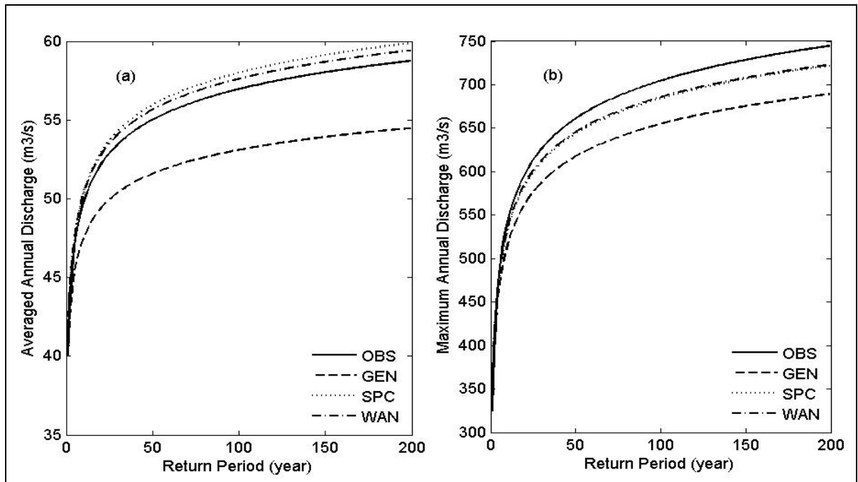
Figure 1.7 Frequencies of mean and maximum annual discharges simulated with the observed, WeaGETS-generated (GEN), and spectral correction (SPC) and Wang and Nathan's (WAN) methods corrected precipitation series.
