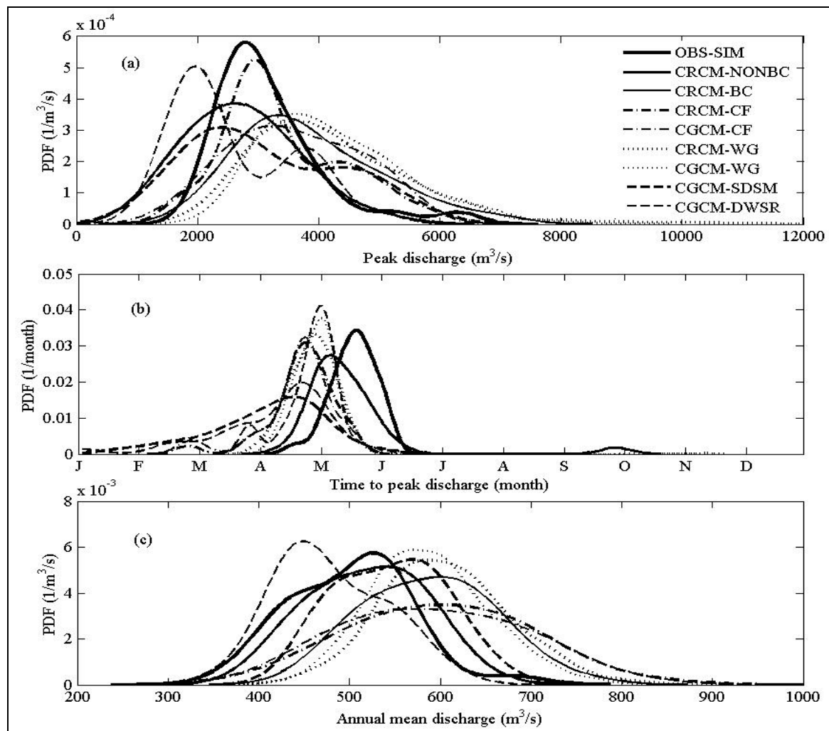
Figure 7.8 Probability density functions (PDF) of (a) peak discharge, (b) time to peak discharge and (c) annual mean discharge for the future (2070-2099) and reference (1970-1999) periods at the Manicouagan 5 river basin.
