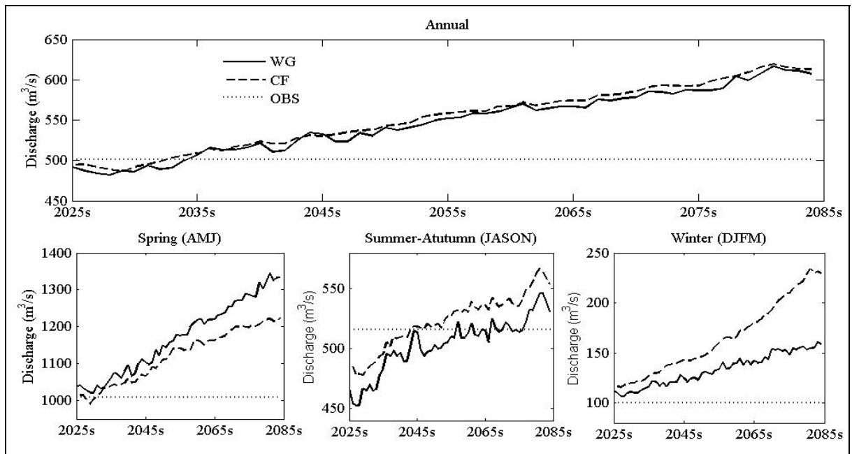
Figure 6.14 Annual and seasonal mean discharge simulated with change factor (CF) and weather generator-based (WG) methods' downscaled precipitation, Tmaxs and Tmin's over the 2025 -2084 period at the Manicouagan 5 river basin. The annual and seasonal mean discharge over the reference period (1970-1999) is shown, for comparison.
