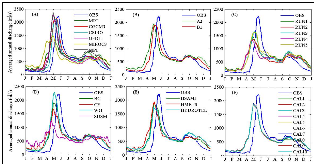
Figure 8.5 Average annual hydrographs for the future (2081-2100) and reference (1971-1990) periods at the Manicouagan 5 river basin. OBS = observed data simulated discharge; CAL1-CAL2 = the set of hydrological model parameters; A=GCMs; B=GGES; C=initial conditions; D=Downscaling methods; E=Hydrology models and F=Hydrology model parameters.
