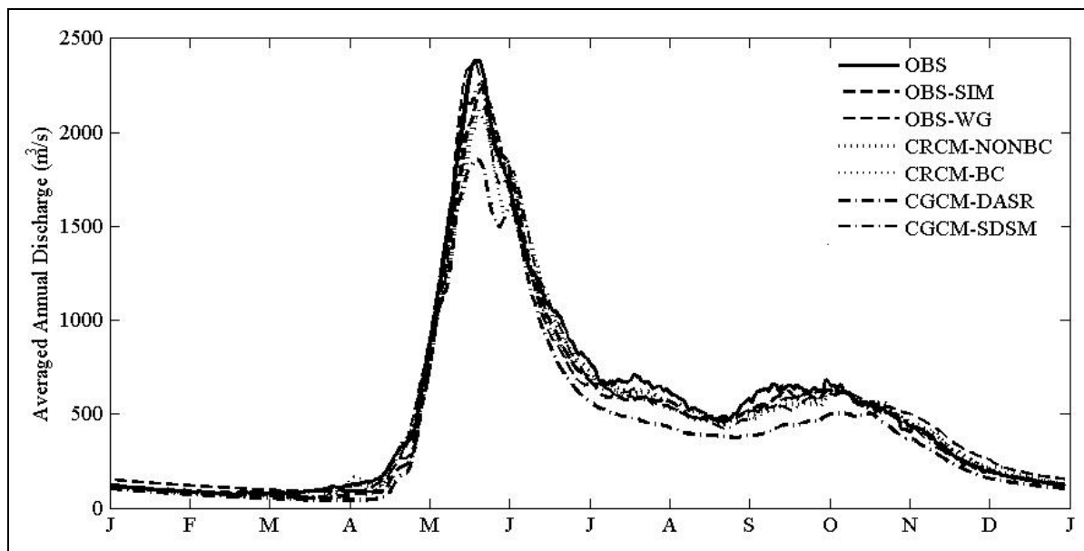
Figure 7.2 Averaged annual hydrographs for the reference period (1970-1999) at the Manicouagan 5 river basin. Observed (OBS), observed weather data simulated (OBS-SIM), and weather generator data simulated (OBS-WG) discharges are also plotted for comparison. See Table 1 for the downscaling method acronyms.
