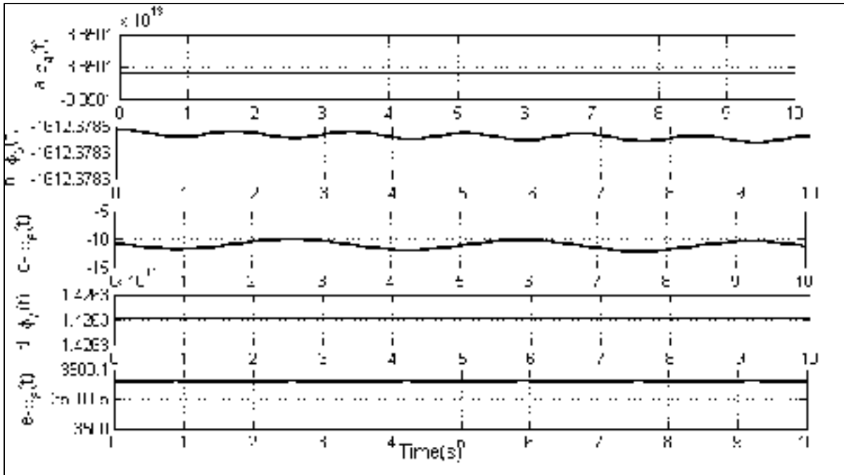
Figure 5.12 Estimated parameters for the adaptive controller \Phi_4 to \Phi_8
