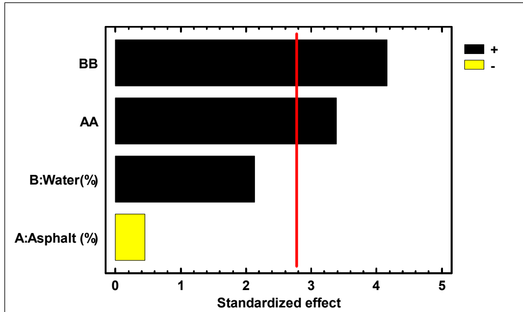
Figure 6.18 Standardized Pareto chart for results of relative moisture retained in WTAT samples (The red line represents the estimated critical F value)
