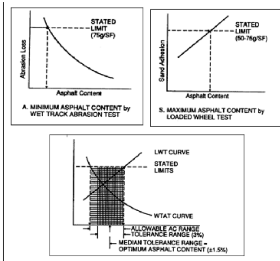
Figure 2.4 Graphical Determination of Optimum Asphalt Content Extracted from Technical Bulletin (ISSA TB 111) International Slurry Seal Associations (2005, p. 2)
