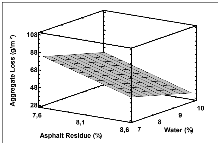
Figure 6.8 Effects of Asphalt Emulsion Residue and Water on Wet Track Abrasion Test (1-Hour Soaked) (Estimates Response)
