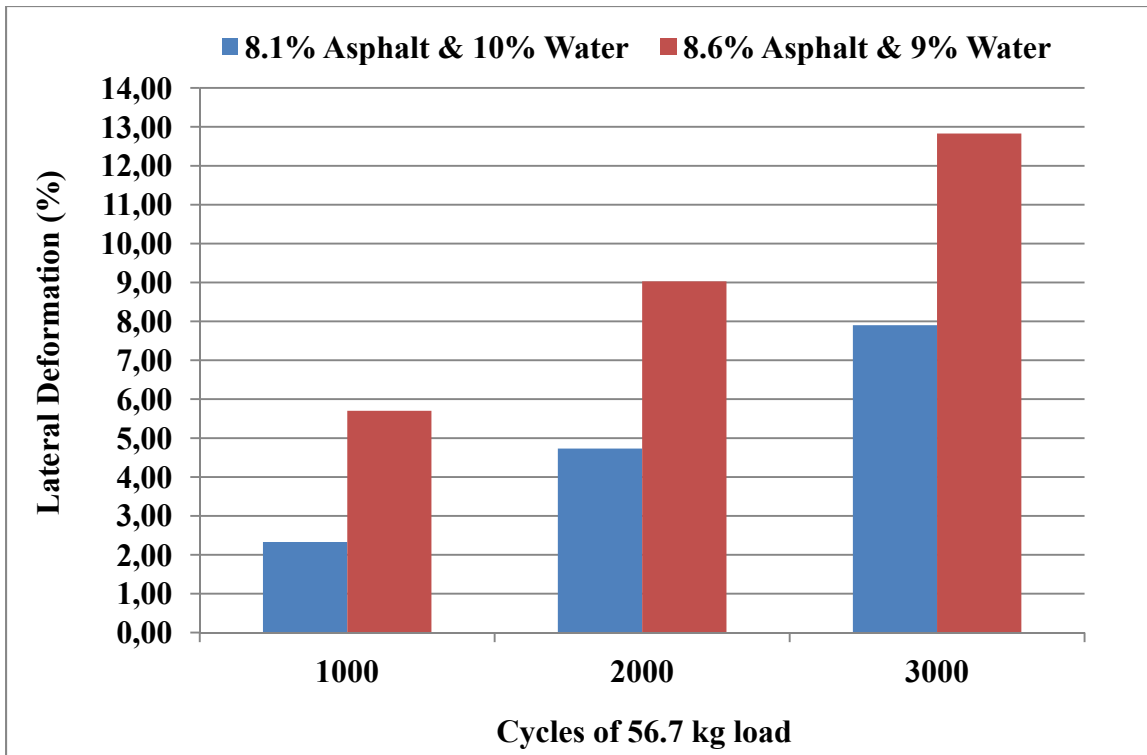
Figure 7.7 Lateral displacement test results, Ray car aggregates
